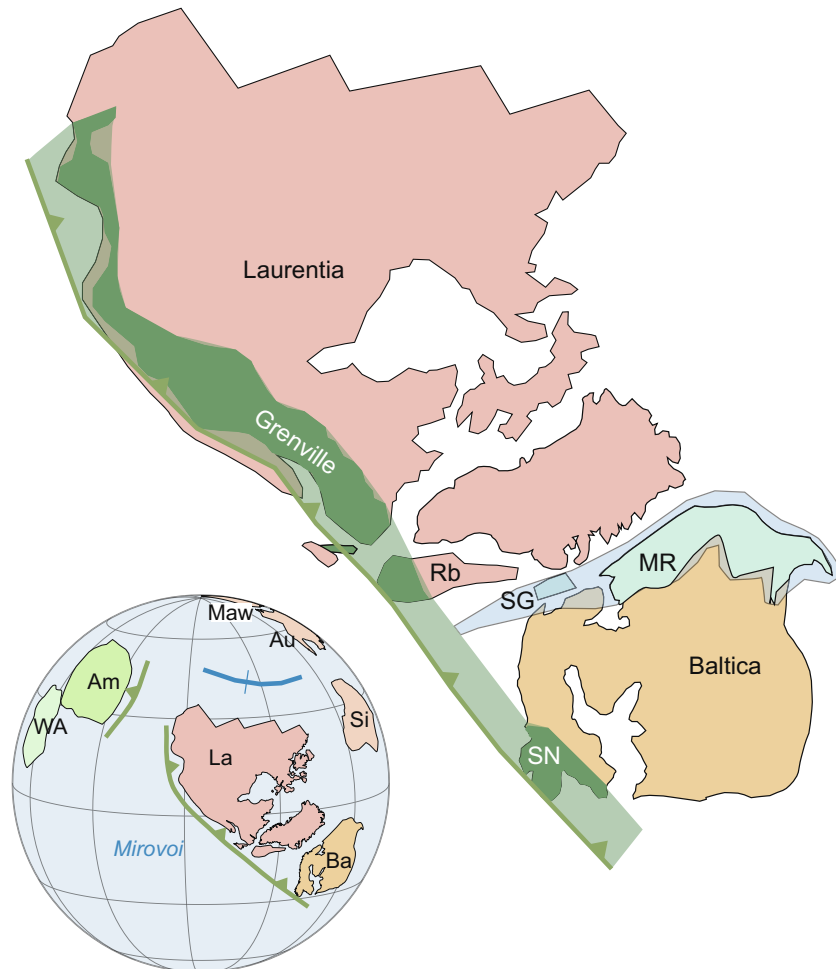
Fig. 1. Laurentia and Baltica at c. 1270 Ma. More detailed reconstruction in lower left shows positions of these and other continents (after Pisarevsky et al., 2014). Abbreviations: Au – Australia; Am – Amazonia; Ba – Baltica; La – Laurentia; MR – Mezen' rift; RB – Rockall Bank; SG – Stoer Group; Si – Siberia; SN – Sveconorwegian Orogen; WA – West Africa.
