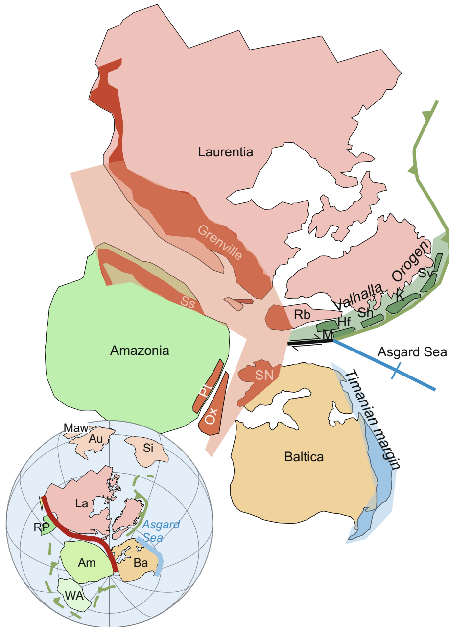
Fig. 2. Laurentia, Baltica and Amazonia at 990 Ma. More detailed reconstruction in lower left shows positions of these and other continents (after Cawood et al., 2016). Abbreviations: Au – Australia; Am – Amazonia; Ba – Baltica; Hf – Hebridean foreland; K – Krummedal succession; La – Laurentia; M – Moine succession; Pt – Putumayo Orogen; Ox – Oaxaquia terrane; Rb – Rockall Bank; RP – Rio de la Plata; Sh – Shetland Islands; Si – Siberia; Sn – Sveconorwegian Orogen; Ss – Sunsas Orogen; Sv – Svalbard; WA – West Africa.
