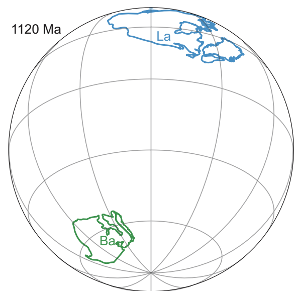
Fig. 4. Reconstruction of Laurentia and Baltica at ca. 1120 Ma (after Pisarevsky, 2016) based on the Salla Dyke paleopole (Salminen et al., 2009). Laurentia is rotated to absolute framework by 70.03° clockwise around Euler pole at 36.27°N, 102.34°W. Baltica is rotated to Laurentia by 121.53° clockwise around Euler pole at 24.65°N, 50.49°W.
