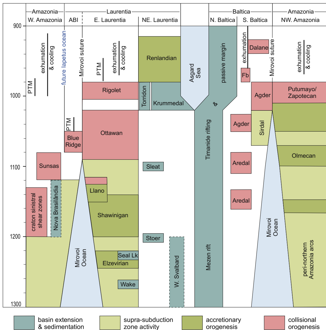
Fig. 3. Schematic time-stratigraphic plot of key late Mesoproterozoic to early Neoproterozoic events along the west and north margins of Amazonia, east and northeast Laurentia, and north and south Baltica. See text for discussion and sources of data. Abbreviations: ABI – Appalachian basement inliers; PTM – post-tectonic magmatism; Wake – Wakeham.
