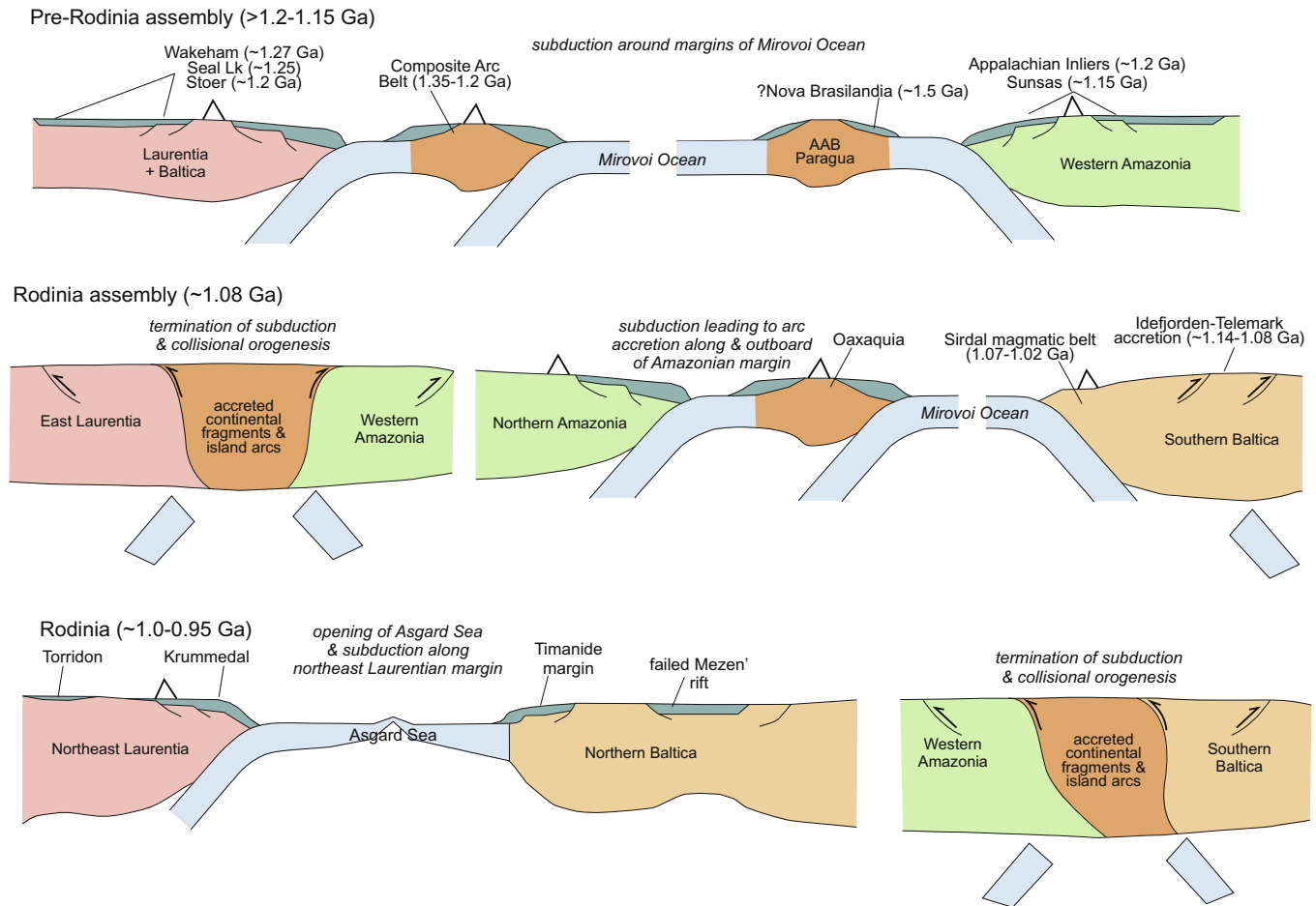
Fig. 5. Series of schematic cross sections between Laurentia, Baltica and Amazonia for the periods pre-Rodinia assembly (>1.2–1.15 Ga), during Rodinia assembly (~1.08 Ga), and for the assembled Rodinia (~1.0–0.95 Ga).
