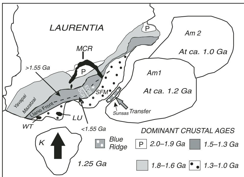
Figure 11. Schematic map of Laurentia showing some major crustal provinces and the proposed collision of the Kalahari craton (K) with the Llano uplift–west Texas area (LU, WT) at ca. 1.25 Ga and Amazonia (Am1 and Am2) with eastern Laurentia at ca. 1.2–1.0 Ga. The arrow pointing the Blue Ridge toward the southeastern Laurentian margin represents the transfer of Amazonian crust to Laurentia. The heavy dashed line separates regions with T_{DM} > 1.55 Ma from those with T_{DM} < 1.55 Ma as indicated. MCR—Midcontinent Rift; P—Penokean Province; SGR—Southern granite-rhyolite province; EGR—Eastern granite-rhyolite province; SFM—St. Francois Mountains (modified from Karlstrom et al., 2001; Loewy et al., 2003; Tohver et al., 2004).
