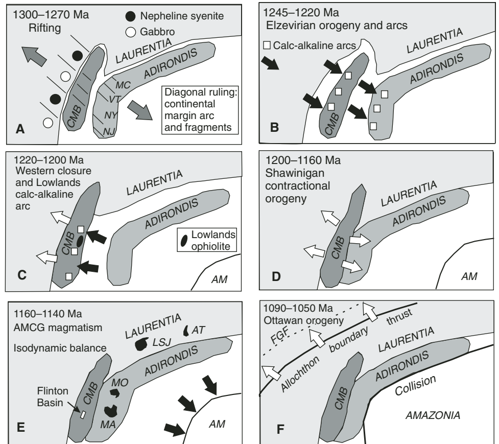
Figure 7. Schematic panel diagram summarizing the distribution and interaction of various segments of northeastern North America during the interval ca. 1300–1050 Ma, encompassing the rifting, opening, and closing of the Central metasedimentary belt (CMB) and the Ottawa collision with Amazonia. Blocky black arrows indicate the polarity of subduction. Blocky open arrows indicate direction of thrusting. Blocky gray arrows represent extension. The model is derived, in part, from Gower (1996), who proposed the term Adirondis to include crust that was rifted from Laurentia at ca. 1.4–1.3 Ga and reattached by collision ca. 1.2–1.0 Ga. As defined here, Adirondis also includes crust of Mauricie (Quebec), Adirondack, and northern Appalachian Mesoproterozoic crust to as far south as the New Jersey Highlands. Also included is Grenvillian-age crust currently buried beneath Paleozoic strata south of the St. Lawrence River. See text for details. Note that Amazonia is inferred to have remained south of the Adirondis region until ca. 1090 Ma, but its regional plate motion is thought to have helped promote closure of the Central metasedimentary belt rift and the Shawinigan collision. Abbreviations: AM—Amazonia; AT—Atikokan River anorthosite; FSG—future Grenville Front; LSJ—Lac St. Jean anorthosite; MA—Marcy anorthosite; MC—Mauricie area, Quebec; MO—Morin anorthosite; NJ—New Jersey; NY—New York; VT—Vermont.
