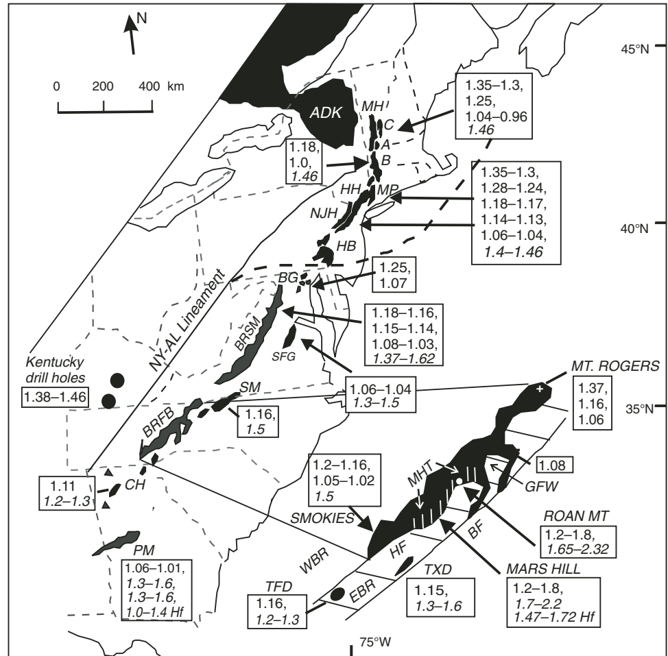
Figure 9. Generalized map of the eastern United States showing Mesoproterozoic massifs in black and their ages in boxes ( T_{DM} in italics). Age references are given in text (Mesoproterozoic Appalachian Inliers section). New York (NY)–Alabama (AL) Lineament is a candidate for a Grenvillian suture zone (Zeitz and, 1978). ADK—Adirondacks; B—Berkshires; BF—Brevard fault zone; BG—Baltimore gneiss dome complex; EBR—Eastern Blue Ridge; BF—Brevard fault; BRFB—Blue Ridge French Broad massif; BRSM—Blue Ridge Shenandoah massif; CH—Corbin Hill; G—Goochland terrane; GMT—Green Mountains; GFW—Grandfather Mountain window; HF—Hayesville fault; HB—Honey Brook uplands; HH—Hudson Highlands; MHT—Mars Hill terrane (vertical white lines); MP—Manhattan Prong; NJH—New Jersey Highlands (Reading Prong); PM—Pine Mountain uplift; TFD—Tallulah Falls Dome; TXD—Toxaway Dome; WBR—western Blue Ridge. The dashed boundary represents the possible eastern limit of Laurentia at ca. 1.2 Ga (modified from Tollo et al., 2006; Carrigan et al., 2003).
