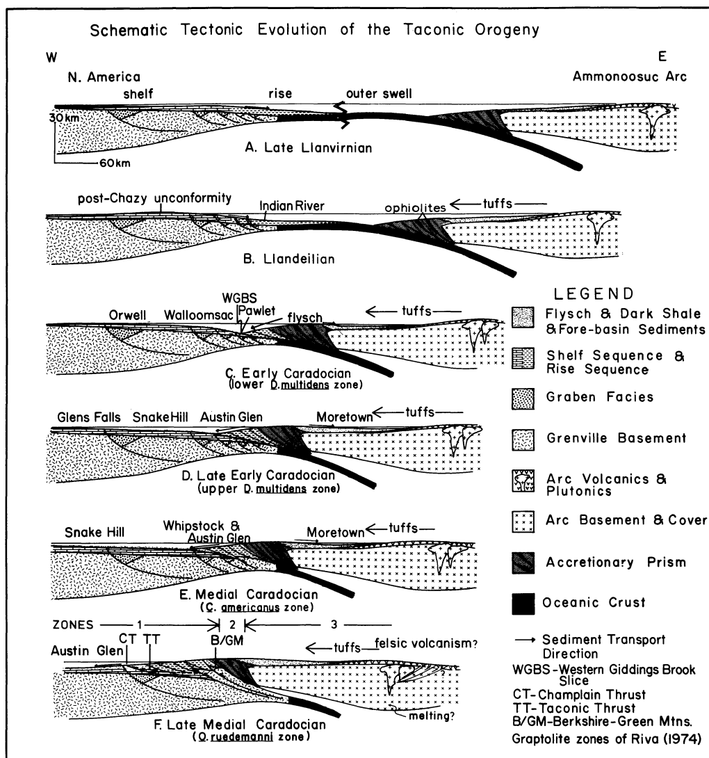
Fig. 4.—Sequential tectonic cross-sections for the Taconic Orogeny in New England. See text for further discussion.
