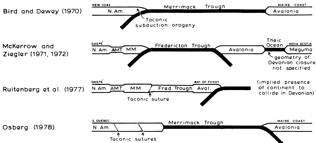
FIG. 1.—Plate tectonics of the Northern Appalachians as visualized by various workers. Cross sections show plate boundary conditions leading up to the Acadian Orogeny; geographic names at left and right locate ends of sections. Other models, not illustrated, include those of Rast and Stringer (1980), Poole (1976), Williams (1978), Robinson and Hall (1979), and Ludman (1981).
