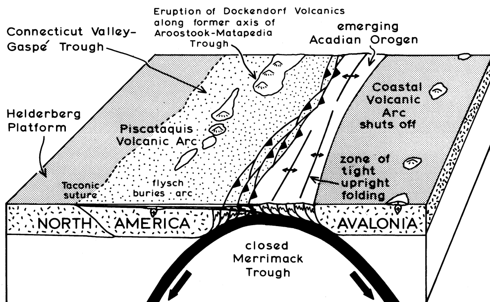
FIG. 6.—Proposed reconstruction of the Acadian Orogen during early Devonian times, near the start of collision between the two accretionary prisms. The west vergent Avalonian prism overthrust its counterpart on the North American side of the ocean, resulting in rapid burial of the Piscataquis Volcanic Arc and the Connecticut Valley-Gaspé Trough beneath a great wedge of easterly-derived flysch. Ornament as in figure 5.
