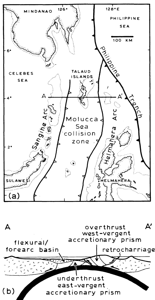
FIG. 4.—(A) Map and (B) cross section of the Molucca Sea collision zone, Indonesia, from Hamilton (1978) and Moore et al. (1981).
