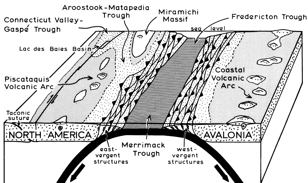
FIG. 5.—Proposed reconstruction of the Acadian Orogen in late Silurian times, showing a contracting Merrimack-Fredericton Ocean (horizontal lines) flanked by oppositely verging subduction zones and corresponding accretionary prisms. Emergent terranes are shown in white, included the Coastal and Piscataquis Volcanic Arcs, Miramichi Massif, and unlabelled high ground over the Taconic suture zone corresponding to “Appalachia” of Boucot (1968). Fine stippling indicates shallow marine deposition; coarser stippling shows areas of deeper water sedimentation, as in the Aroostook-Matapedia Trough.
