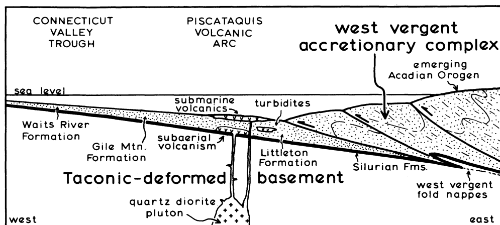
FIG. 7.—Illustration of the effects of downflexing of the North American margin beneath the weight of the advancing Avalonian accretionary complex. Heretofore subaerial and shallow marine conditions in the Piscataquis belt were replaced by deep water flysch sedimentation and sporadic submarine volcanism. Transport of the early west vergent fold nappes of Thompson et al. (1968) is here attributed to shear stress imposed by the overthrusting accretionary complex.
