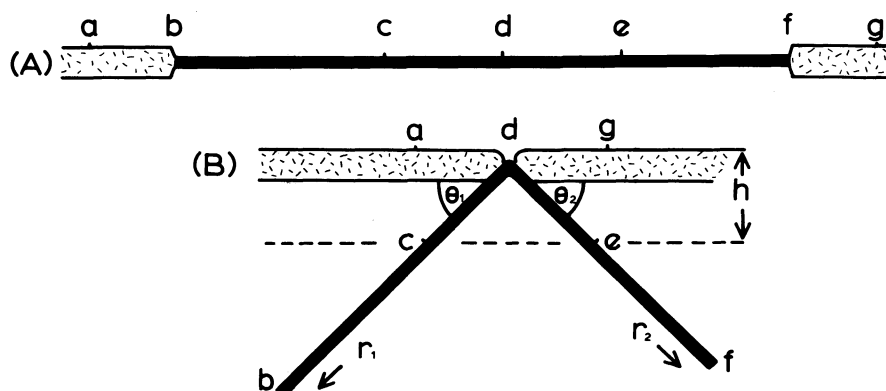
FIG. 3.—Method of estimating the original width of the Merrimack Trough (A), from the geometry and duration of subduction (B) inferred from geologic data. Terms in Equation 1 (see text) are equated with lengths in figure as follows: bf = w ; bc = r_1 t_1 ; cd = h \sin \theta_1 ; de = h \sin \theta_2 ; ef = r_2 t_2 . Points a and g are loci of arc volcanism.
