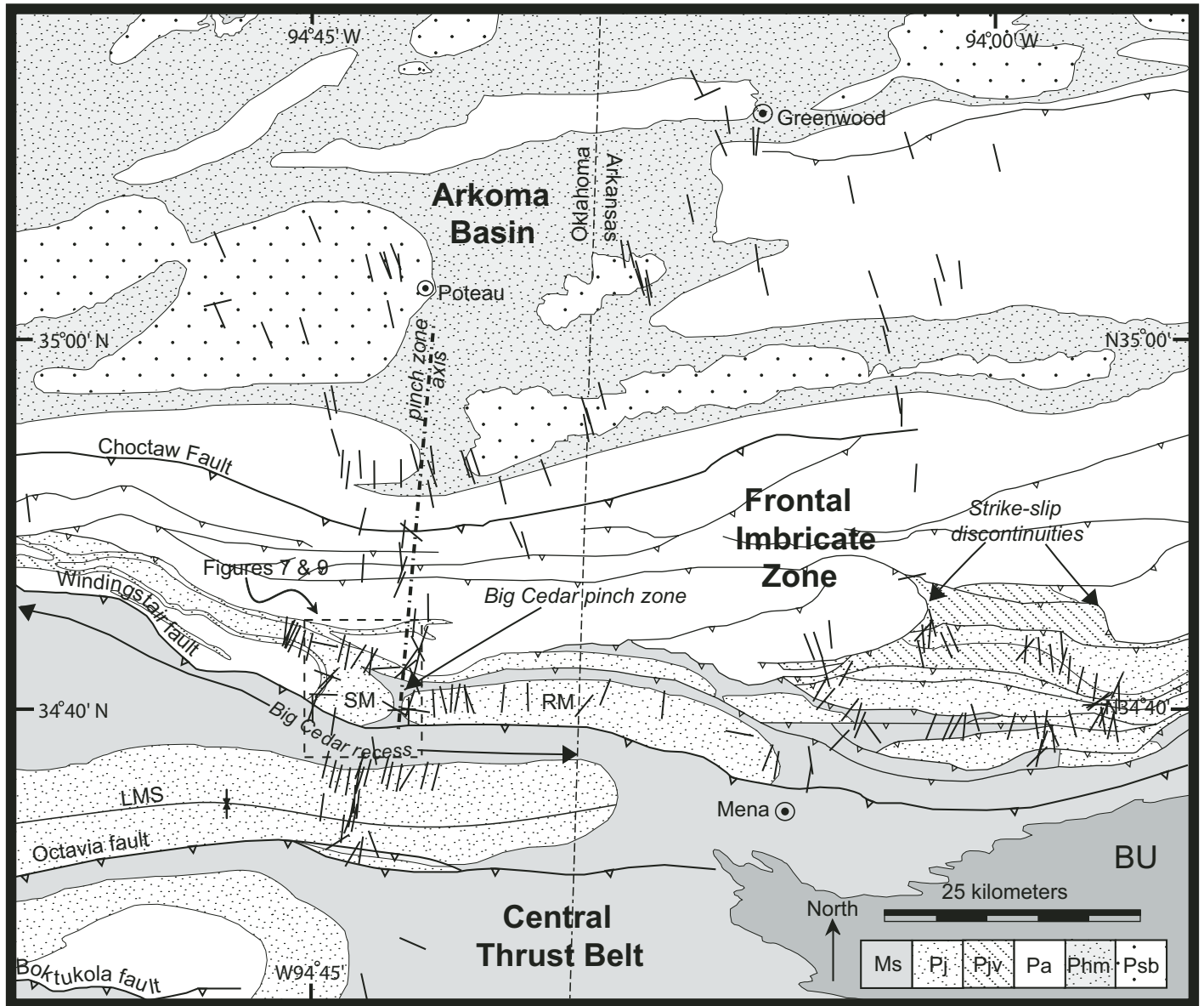
Figure 3. Simplified geological map of the central Ouachita fold-and-thrust belt and Arkoma Basin with mean joint azimuth of the most-frequent joint set plotted for selected outcrops. Major thrust faults (Boktukola, Octavia, Windingstair, Choctaw) are traced with bold lines. Imbrications in the frontal imbricate zone are traced with lighter lines. Formation symbols are: Ms—Mississippian Stanley Group; Pj—Pennsylvanian (Morrowan) Jackfork Group; Pjv—Pennsylvanian (Morrowan) Johns Valley Formation; Pa—Pennsylvanian (Atokan) Atoka Formation; Phm—Pennsylvanian (Desmoinesian) Hartshorne and McAlester Formations; Psb—Pennsylvanian (Desmoinesian) Savanna and Boggy Formations. See Figure 2 for the location of the study area. LMS—Lynn Mountain syncline; SM—Simmons Mountain syncline; RM—Rich Mountain syncline; BU—Benton uplift.
