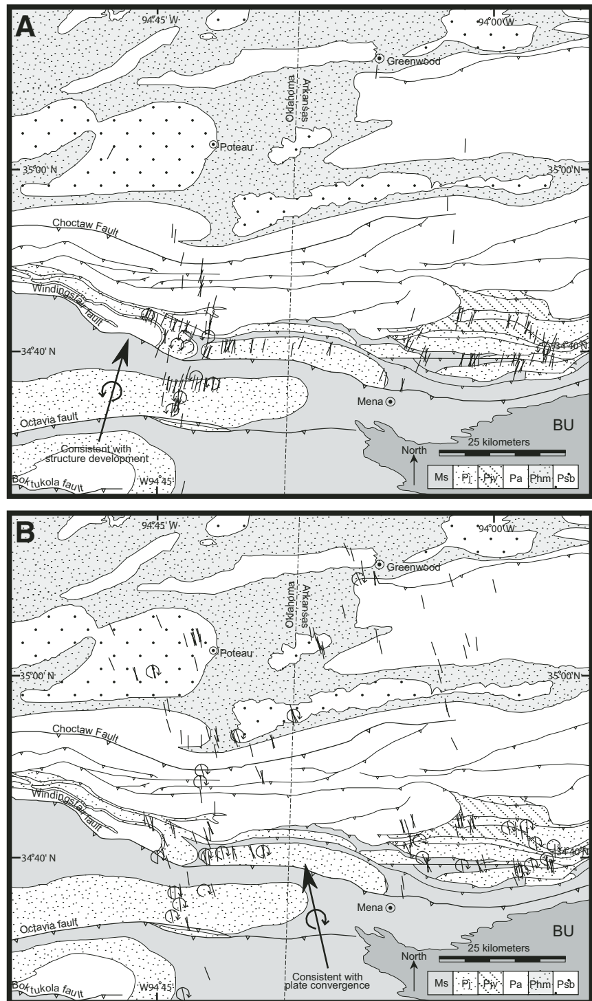
Figure 5. Summary of fringe cracks, cross-fold joints, and tectonic compression directions indicated by joints in the Ouachita Mountains. The display illustrates how the NNE and NNW joint sets can be distinguished by fringe crack development as well as by orientation. The NNE joints formed earlier in Atoka and older rocks. The NNW set formed later and is found in the Desmoinesian Boggy Formation and all older Carboniferous strata. Formations are: Ms—Stanley Group; Pj—Jackfork Group; Pjv—Johns Valley Formation; Pa—Atoka Formation; Phm—Hartshorne and McAlester Formations; Psb—Savanna and Boggy Formations; BU—Benton uplift. A simplified pattern of joints and fringe cracks is shown. (A) Older-stage NNE-striking joints and anticlockwise fringe cracks. (B) Younger-stage NNW-striking joints and clockwise fringe cracks.
