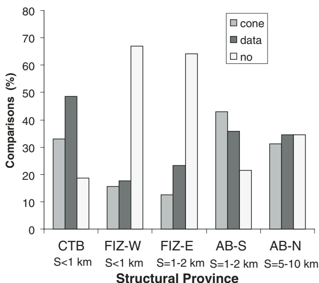
Figure 12. Station to station continuity of joint sets in three structural provinces of the Ouachita belt. Plot illustrates that even with greater spacing between outcrops in the Arkoma Basin (AB), joint orientations remain consistent. Also, frontal imbricate zone (FIZ) joints rarely have continuous orientations, even at closely spaced outcrops. “Cone” indicates that the 95% confidence cones for joint sets at two adjacent stations overlap; “data” indicates that the data range for joint sets at two adjacent stations overlap; and “no” indicates that there is no data range overlap for joint sets at two adjacent stations. Abbreviations: CTB—central thrust belt; FIZ-W—western frontal imbricate zone (Oklahoma); FIZ-E—eastern frontal imbricate zone (Arkansas); AB-S—southern Arkoma Basin; AB-N—northern Arkoma Basin; S—(average) spacing between outcrops.
