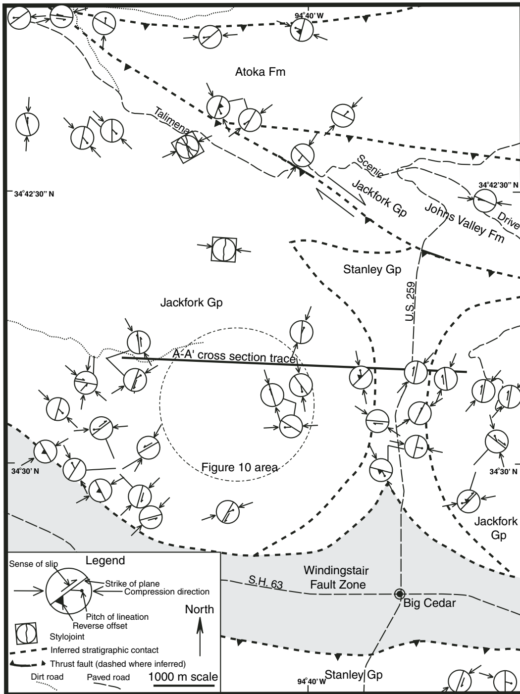
Figure 9. Faults near the Big Cedar pinch zone, the strikes of which are oblique to the primary transport direction. Interpreted compression directions are parallel to the lineation, or, if only a sense of slip was available, they are parallel to the friction angle. A stylojoint is a vertical joint, the surface of which was later stylolitized. The compression direction on the stylojoints is inferred from the stylolitic cleavage. Approximate stratigraphic contacts are shown as dashed lines. Approximate fault contacts are shown with toothed dashed lines. Cross-section A-A' is shown on Figure 8. The highly deformed area around the Windingstair fault is shaded. The area enclosed by the dashed circle contains the joint data plotted in Figure 10. S.H.—state highway.
