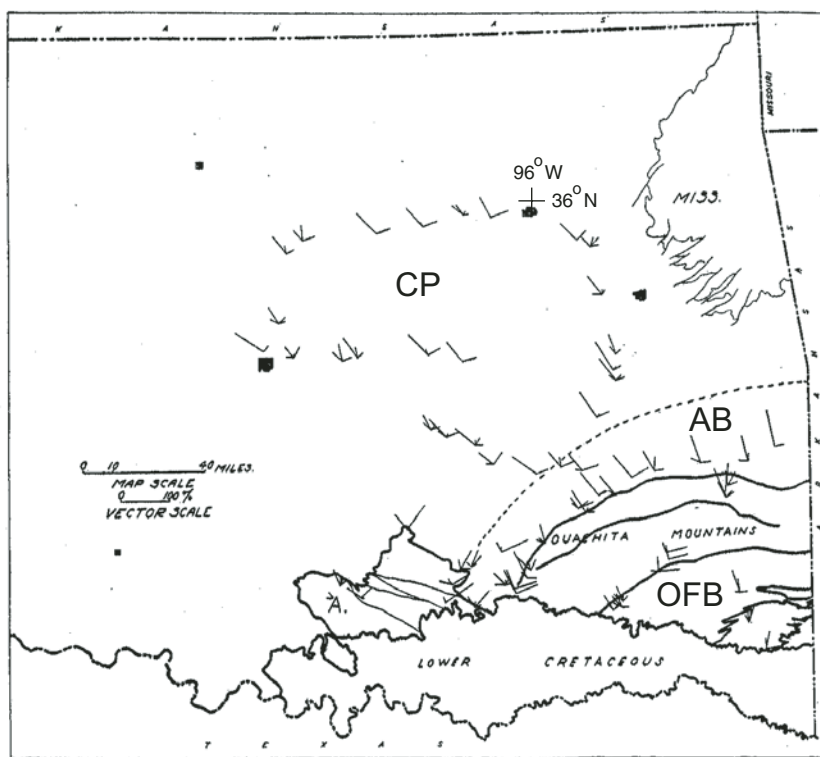
Figure 1. Melton's (1929) map of joint patterns in the Central Plains (CP), Arkoma Basin (AB), and Ouachita fold-and-thrust belt (OFB).
