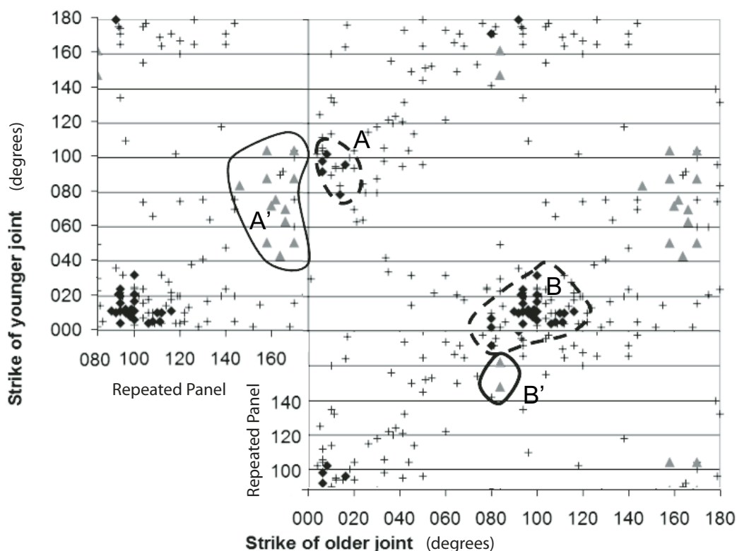
Figure 6. Age relationships among joints in the three provinces. There are two clusters (A–A' and B–B') of orthogonal joints. Joints in the Arkoma Basin (A', B') are offset in an anticlockwise direction from joints in the central thrust belt (A, B). In the central thrust belt, the E-W joint set is older, whereas it is younger in the Arkoma Basin. These data suggest that the cross-fold joints propagated during anticlockwise stress rotation prior to the onset of folding in the Arkoma Basin. Data from the central thrust belt are plotted as diamonds. Data from the frontal imbricate zone are plotted as crosses. Data from the Arkoma Basin are plotted as triangles. Strikes are normalized to the east component.
