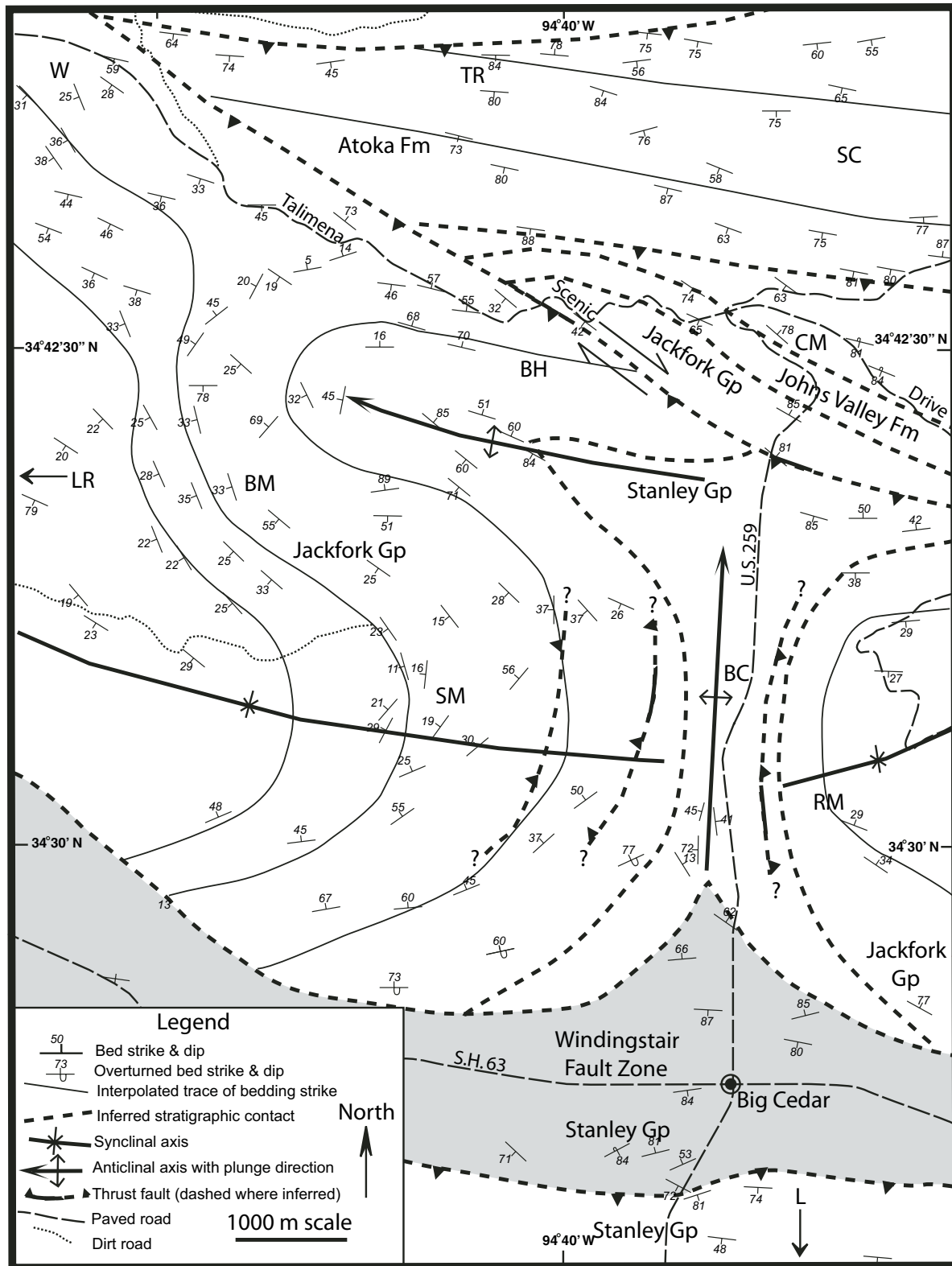
Figure 7. Simplified geological map of the structure of the Big Cedar pinch zone. Bedding attitudes are shown with fine lines interpolating bedding strike between outcrops. Major anticlinal and synclinal hinges are also plotted. Abbreviations: L—Lynn Mountain syncline; RM—Rich Mountain syncline; SM—Simmons Mountain syncline; BC—Big Cedar pinch zone; BM—Bowman Mountain; LR—Lenox Ridge; BH—Billy Hill; CM—Coon Mountain; TR—Tram Ridge; W—Windingstair Mountain; Gp—Group; S.H.—state highway. Approximate stratigraphic contacts are shown as dashed lines. Approximate fault contacts are shown with toothed dashed lines. The highly deformed area around the Windingstair fault is shaded.
