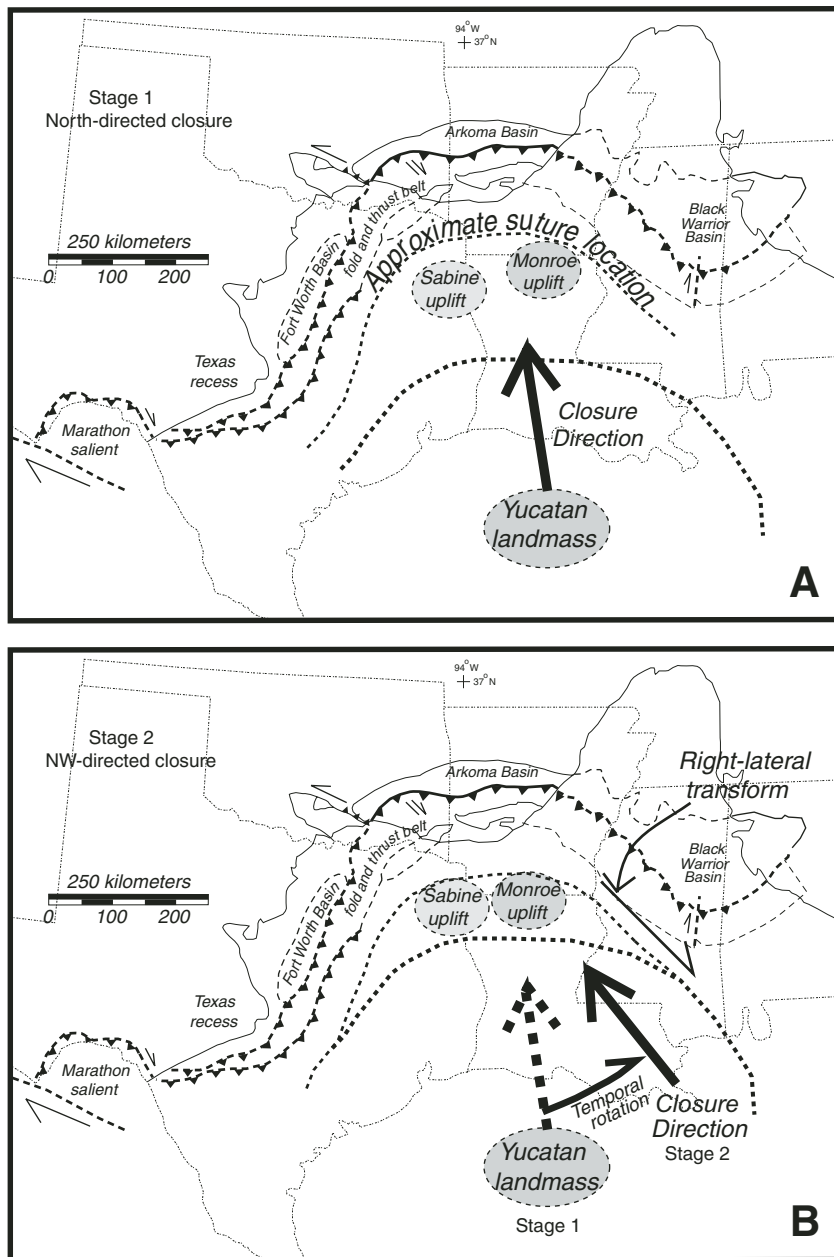
Figure 13. Two-stage tectonic evolution of the Ouachita salient. Map is after Pindell (1985) and Viele and Thomas (1989). (A) First stage of the Ouachita orogeny characterized by northward S_H during closure of the Sabine/Monroe terrane. (B) After the docking of the Sabine/Monroe terrane, continued closure of the Yucatan landmass forms the Mississippi slate belt (right-lateral transform) and NW-directed S_H .
