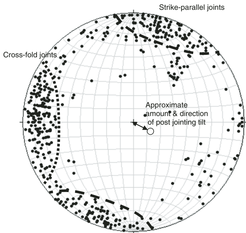
Figure 10. Equal-area stereonet of poles to cross-fold and fold-parallel joints measured in the Simmons Mountain syncline. Figure also shows the \sim 15^\circ of NW displacement of the two joint sets after their formation. NW displacement occurred with the development of the Big Cedar pinch zone. See Figure 9 for the area in which joints in this plot were measured.
