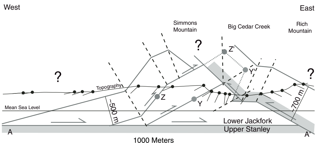
Figure 8. Schematic cross section across the Big Cedar pinch zone. The location of the A–A' line of section is shown on Figure 9. The shaded area is Stanley Group; all other rocks are Jackfork Group. Tadpoles indicate the apparent dip of bedding to the east or west. The approximate trace of the overturned anticline before it was cut off by the west-verging fault is shown with a fine-dashed line. Fold hinges are coarse-dashed lines. Points Z' and Y' would have unfolded to approximately the location of points Z and Y. Question marks indicate that no attempt was made to constrain the roof geometry in those areas.
