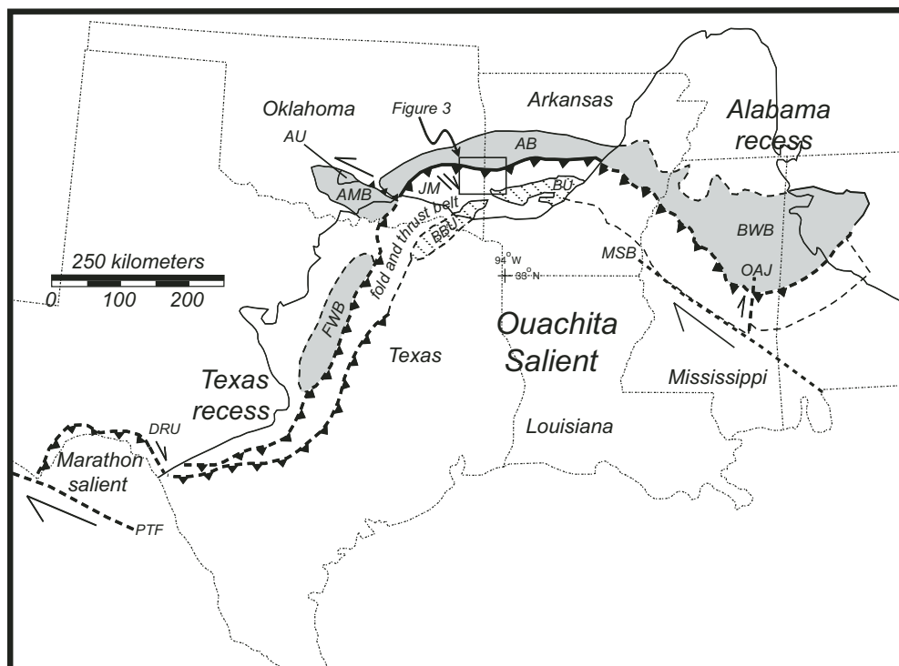
Figure 2. Tectonic map of the Ouachita salient showing zones of strike-slip displacement during the Ouachita orogeny. Background map is after Viele and Thomas (1989). Foreland basins are shaded; Broken Bow and Benton uplifts are stippled. Abbreviations: AB—Arkoma Basin; BWB—Black Warrior Basin; BU—Benton uplift; BBU—Broken Bow uplift; FWB—Fort Worth Basin; AMB—Ardmore/Marietta Basin (sinistral slip from Granath, 1989; Pindell, 1985, indicates the slip is dextral); AU—Arbuckle uplift; JM—Jackfork Mountain (dextral slip from Miser et al., 1954; Arbenz, 1989); MSB—Mississippi slate belt (dextral slip from Pindell, 1985); OAJ—Ouachita-Appalachian juncture (dextral slip from Hale-Erlich and Coleman, 1993); DRU—Devil's River uplift (dextral slip from Pindell, 1985); PTF—Pedregosa Trough fault system (dextral slip from Pindell, 1985).
