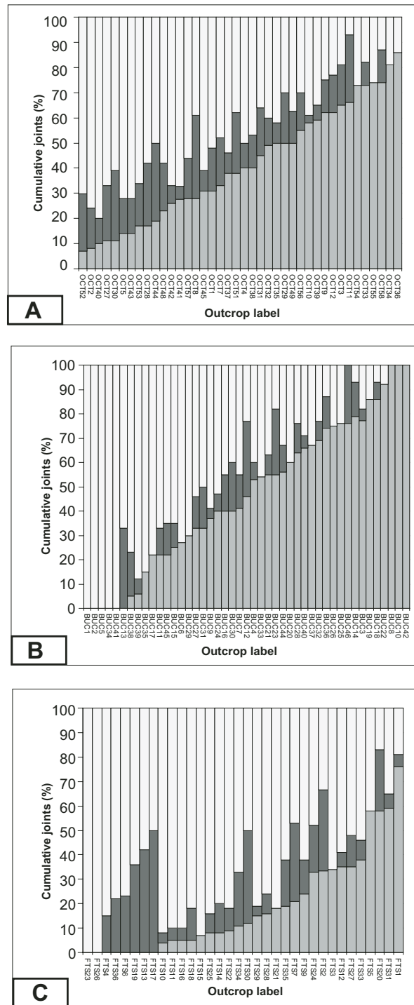
Figure 11. Graphs of the results of transforming cross-fold joints to prefold coordinates by station in Ouachita belt. In the central thrust belt and frontal imbricate zone, about half of joints formed before folding, whereas Arkoma Basin joints primarily formed after folding. The gray bars indicate joints that are steepened by the transformation of joints to prefold coordinates. The dark gray bars represent joints that are marginally steepened ( <2^\circ ) by the transformation of joints to prefold coordinates. Together, black and gray compose prefolding joints as discussed in the text. The white bars represent joints made shallower by the transformation of joints to prefold coordinates and are referred to as postfolding joints in the text. (A) Outcrops from the central thrust belt. (B) Outcrops from the frontal imbricate zone. (C) Outcrops from the Arkoma Basin.
