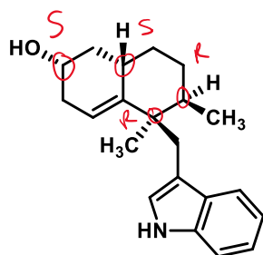
Polyathanol
