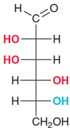
D-Mannose
