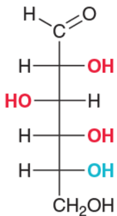
D-Glucose
