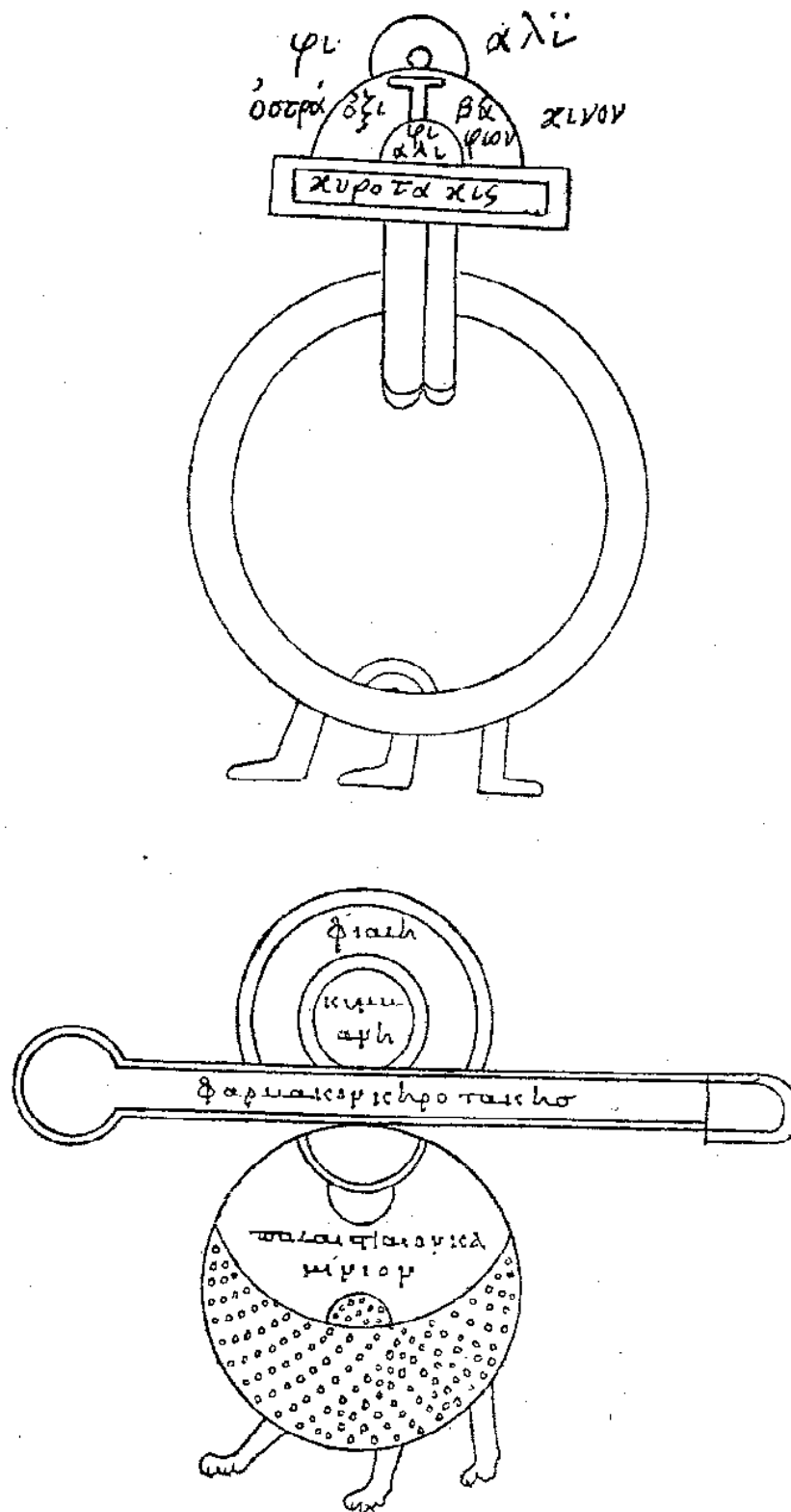
FIG. 6.—TWO TYPES OF THE MORE COMPLEX KEROTAXIS APPARATUS FROM THE MS. MARC. 299. CONJECTURAL RECONSTRUCTIONS ARE GIVEN IN FIG. 7.
