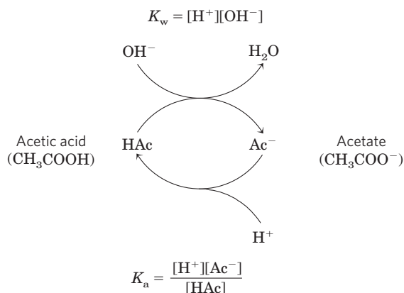
FIGURE 2–19 The acetic acid–acetate pair as a buffer system. The system is capable of absorbing either H^+ or OH^- through the reversibility of the dissociation of acetic acid. The proton donor, acetic acid (HAc), contains a reserve of bound H^+ , which can be released to neutralize an addition of OH^- to the system, forming H_2O . This happens because the product [H^+][OH^-] transiently exceeds K_w ( 1 \times 10^{-14} M^2 ). The equilibrium quickly adjusts to restore the product to 1 \times 10^{-14} M^2 (at 25 °C), thus transiently reducing the concentration of H^+ . But now the quotient [H^+][Ac^-]/[HAc] is less than K_a , so HAc dissociates further to restore equilibrium. Similarly, the conjugate base, Ac^- , can react with H^+ ions added to the system; again, the two ionization reactions simultaneously come to equilibrium. Thus a conjugate acid-base pair, such as acetic acid and acetate ion, tends to resist a change in pH when small amounts of acid or base are added. Buffering action is simply the consequence of two reversible reactions taking place simultaneously and reaching their points of equilibrium as governed by their equilibrium constants, K_w and K_a .
