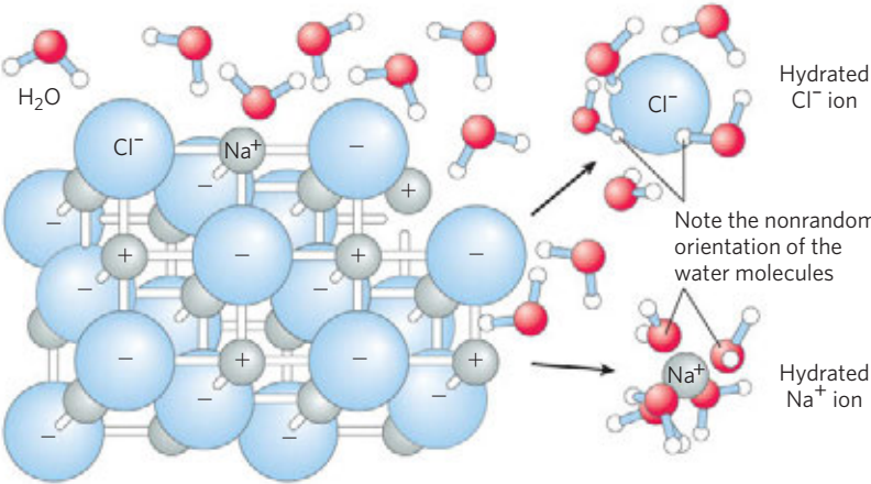
FIGURE 2-6 Water as solvent. Water dissolves many crystalline salts by hydrating their component ions. The NaCl crystal lattice is disrupted as water molecules cluster about the Cl − and Na + ions. The ionic charges are partially neutralized, and the electrostatic attractions necessary for lattice formation are weakened.
