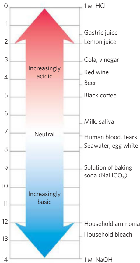
FIGURE 2-15 The pH of some aqueous fluids.
