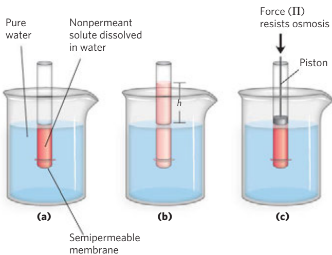
FIGURE 2-12 Osmosis and the measurement of osmotic pressure.
