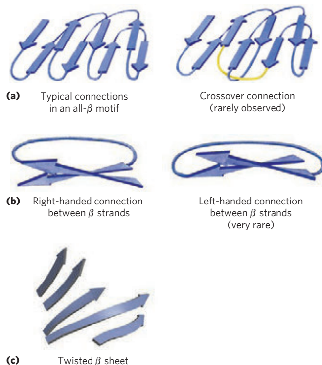
FIGURE 4-20 Stable folding patterns in proteins. (a) Connections between \beta strands in layered \beta sheets. The strands here are viewed from one end, with no twisting. Thick lines represent connections at the ends nearest the viewer; thin lines are connections at the far ends of the \beta strands. The connections at a given end (e.g., near the viewer) rarely cross one another. An example of such a rare crossover is illustrated by the yellow strand in the structure on the right. (b) Because of the right-handed twist in \beta strands, connections between strands are generally right-handed. Left-handed connections must traverse sharper angles and are harder to form. (c) This twisted \beta sheet is from a domain of photolyase (a protein that repairs certain types of DNA damage) from E. coli (derived from PDB ID 1DNP). Connecting loops have been removed so as to focus on the folding of the \beta sheet.
