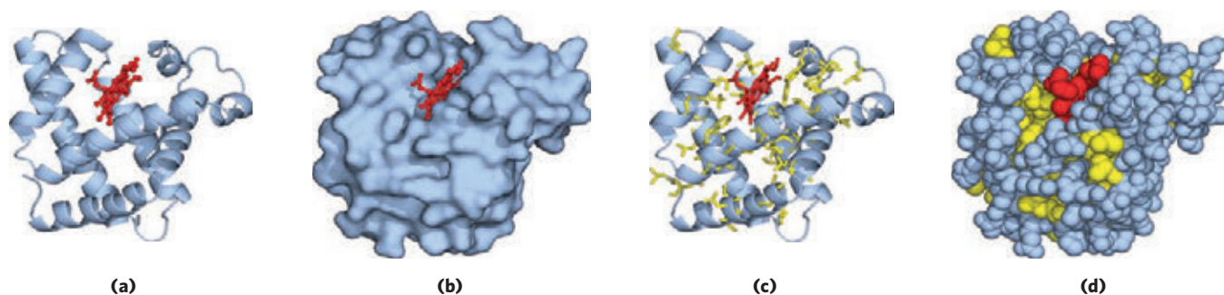
FIGURE 4-16 Tertiary structure of sperm whale myoglobin. (PDB ID 1MBO) Orientation of the protein is similar in (a) through (d); the heme group is shown in red. In addition to illustrating the myoglobin structure, this figure provides examples of several different ways to display protein structure. (a) The polypeptide backbone in a ribbon representation of a type introduced by Jane Richardson, which highlights regions of secondary structure. The \alpha -helical regions are evident. (b) Surface contour
