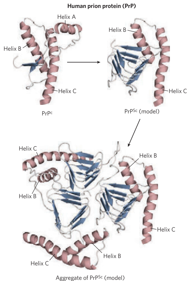
FIGURE 2 Structure of the globular domain of human PrP (PDB ID 1QLX) and models of the misfolded, disease-causing conformation \text{PrP}^{\text{Sc}} , and an aggregate of \text{PrP}^{\text{Sc}} . The \alpha helices are labeled to help illustrate the conformation change. Helix A is incorporated into the \beta -sheet structure of the misfolded conformation.
