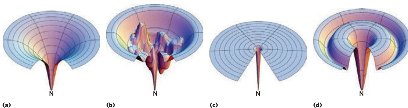
FIGURE 4-29 The thermodynamics of protein folding depicted as free-energy funnels. As proteins fold, the conformational space that can be explored by the structure is constrained. This is modeled as a three-dimensional thermodynamic funnel, with \Delta G represented as depth and with the native structure (N) at the bottom (lowest free-energy point) of the funnel. The funnel for a given protein can have a variety of shapes, depending on the number and types of folding intermediates in the folding pathways. Any folding intermediate with significant stability and a finite lifetime would be represented as a local free-energy minimum—a depression on the surface of the funnel. (a) A simple but relatively wide and smooth funnel represents a protein that has multiple folding pathways (that is, the order in which different parts of the protein fold would be somewhat random), but it assumes its three-dimensional structure with no
