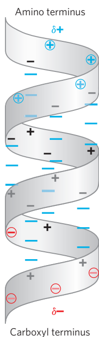
FIGURE 4-5 Helix dipole. The electric dipole of a peptide bond (see Fig. 4-2a) is transmitted along an \alpha -helical segment through the intrachain hydrogen bonds, resulting in an overall helix dipole. In this illustration, the amino and carbonyl constituents of each peptide bond are indicated by + and - symbols, respectively. Non-hydrogen-bonded amino and carbonyl constituents of the peptide bonds near each end of the \alpha -helical region are circled and shown in color.
