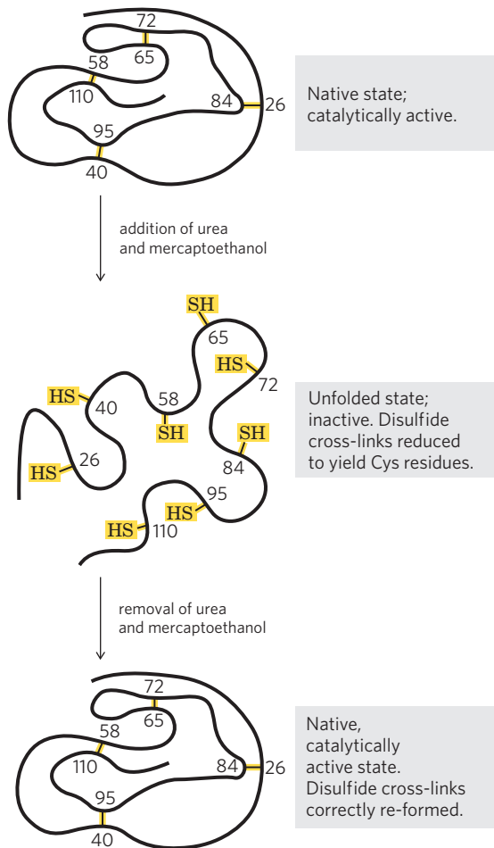
FIGURE 4-27 Renaturation of unfolded, denatured ribonuclease.
