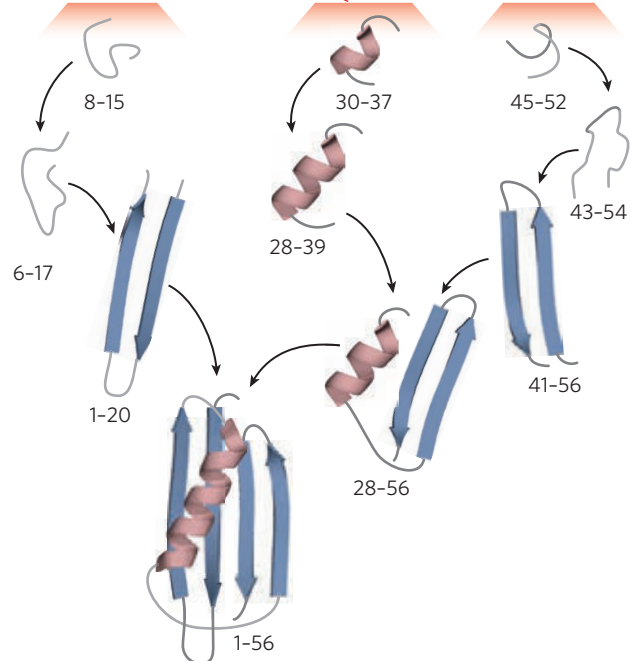
FIGURE 4-28 A protein-folding pathway as defined for a small protein.
