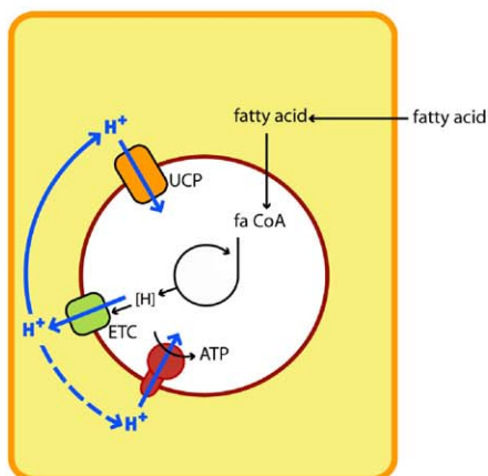
MODEL 1A Basal thermogenesis
