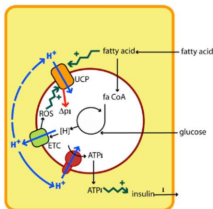
MODEL 3 Regulation of insulin secretion
