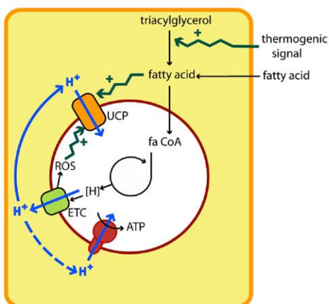
MODEL 1B Inducible thermogenesis
