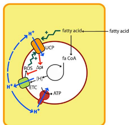
MODEL 2 Attenuation of ROS production
