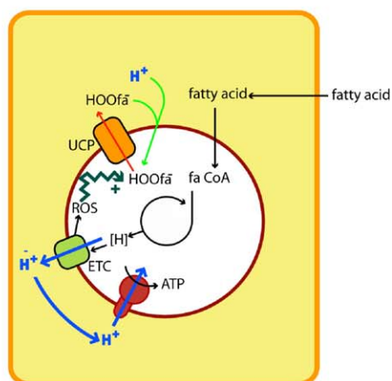
MODEL 4B Fatty acid peroxide export
