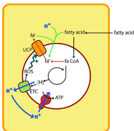
MODEL 4A Fatty acid export
