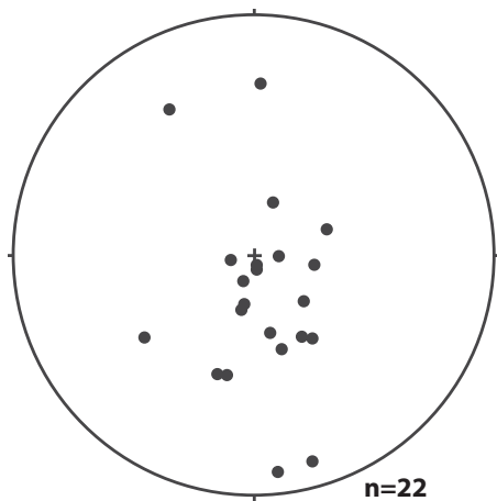
Figure 7. Equal-area lower-hemisphere stereonet for 22 measurements of bulk finite strain from the predominately folded cover sequence in the Valley and Ridge, showing orientations of the long axes for calculated strain ellipses after restoring bedding to horizontal.
