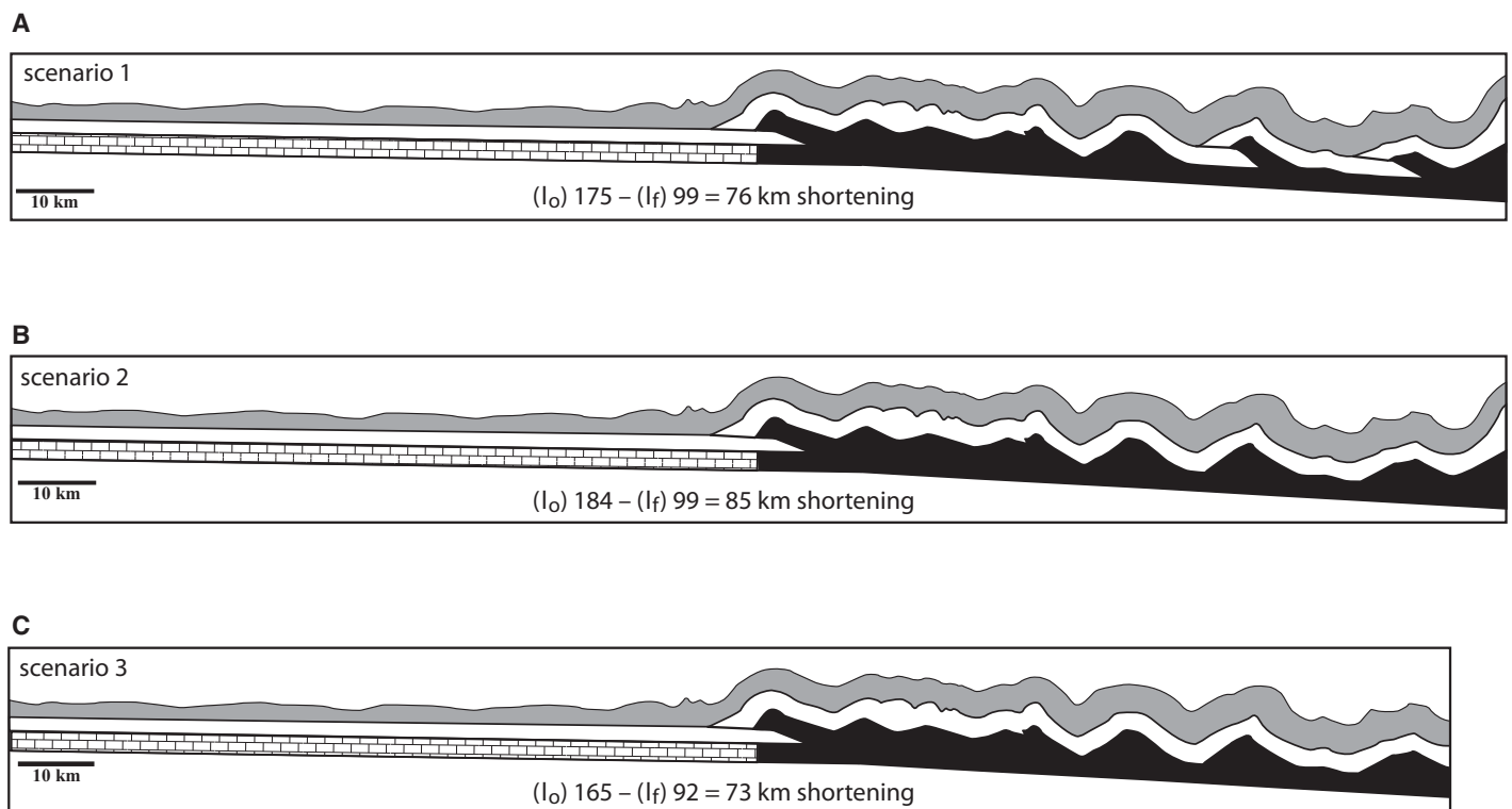
Figure 10. Area-balance calculations for the Cambrian–Ordovician sequence along profile A–A'. Symbols: black shaded area—deformed Cambrian–Ordovician strata; patterned region—undeformed Cambrian–Ordovician strata; white region—strata between the Ordovician Reedsville Formation and the Silurian Wills Creek Formation; gray shaded region—strata above the Silurian Wills Creek Formation; l_0 —undeformed length; l_f —deformed length. (A) Area of repeated Cambrian–Ordovician rocks from our balanced cross section (Plate 1). Note the amount of area highlighted in A is strongly dependent on the kinematic scenario we proposed where two faults (faults 8 and 10 in Plate 1) repeat the Cambrian–Silurian section. (B) Area balance assuming that the décollement in the Ordovician Reedsville Formation (Fig. 3 and Plate 1) always separates folded strata from faulted strata and all space is filled by repeating the Cambrian–Ordovician section. (C) Area balance assuming that the southern limit of the cross section is situated along the axis of the southernmost syncline. Here, the cover rocks suggest 67 km of shortening, while the area balanced Cambrian–Ordovician section indicates 73 km of shortening.
