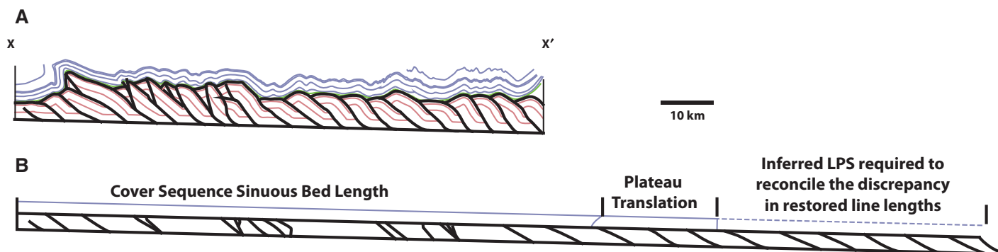
Figure 2. (A) Simplified geologic cross section extending from the southern boundary of the Valley and Ridge physiographic province to the pin line on the Appalachian Plateau. (B) Restored cross section from X–X' highlighting the 28% discrepancy in the restored line lengths between imbricated carbonate sequence and overlying mainly folded strata. Cross section is simplified from Herman (1984). LPS—layer-parallel shortening.
