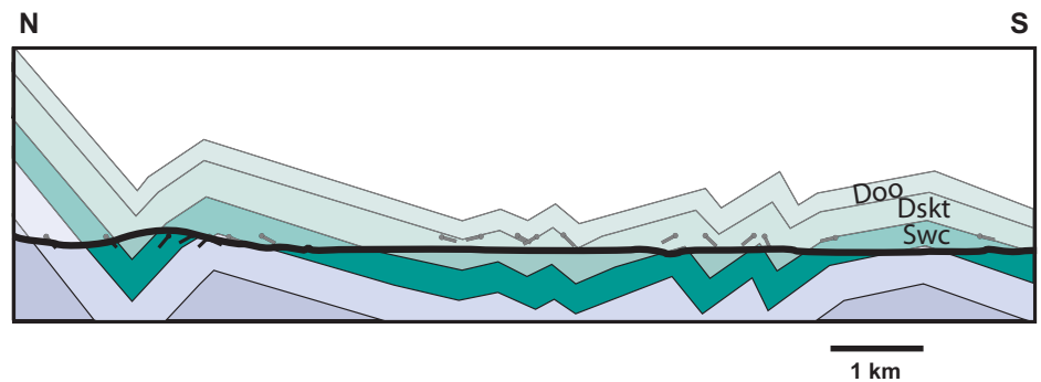
Figure 8. Detailed geologic cross section of second-order folds in the northern Valley and Ridge Province. The line of section is shown in Figure 4, and the stratigraphic color key is in Plate 1.
