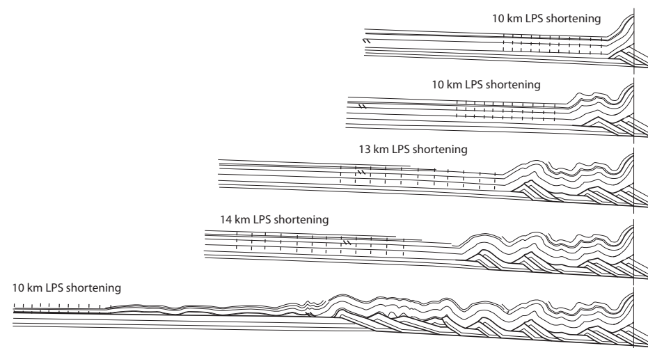
Figure 12. (A) Layer-parallel shortening (LPS) on the Appalachian Plateau is limited to strata above the Silurian Wills Creek Formation. This shortening is linked to early duplex development where two faults cut through the entire Cambrian through Silurian section. (B) LPS immediately precedes folding and only the last LPS (10 km) on the Appalachian Plateau is limited to Silurian and younger strata. In this scenario, the Ordovician Reedsville Formation always separates faulted strata from folded strata, and some LPS (14 km) is accommodated in the Ordovician and younger rocks in the plateau.
