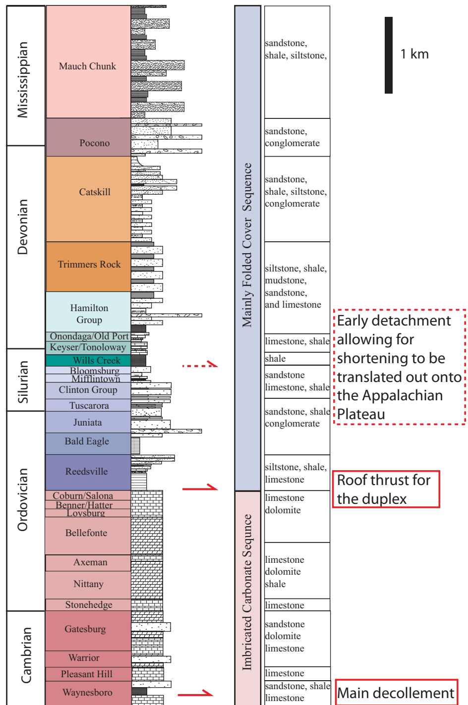
Figure 3. Stratigraphic column for the central Appalachian Valley and Ridge Province (compiled from Ayrton, 1963; Colton, 1963; Hoskins et al., 1963; Sutton, 1963; Gwinn, 1964; Dyson, 1967; Faill and Wells, 1974; Hoskins, 1976; Faill and Nickelsen, 1973, 1977, 1978; Berg and Edmunds, 1979; Wells and Bucek, 1980; Inners, 1981, 1997; Berg et al., 1983, 1993; Epstein, 1986; Edmunds, 1993, 1996). Note that the Ordovician Martinsburg Formation is the Great Valley temporal equivalent to the Reedsville Formation in the Valley and Ridge.
