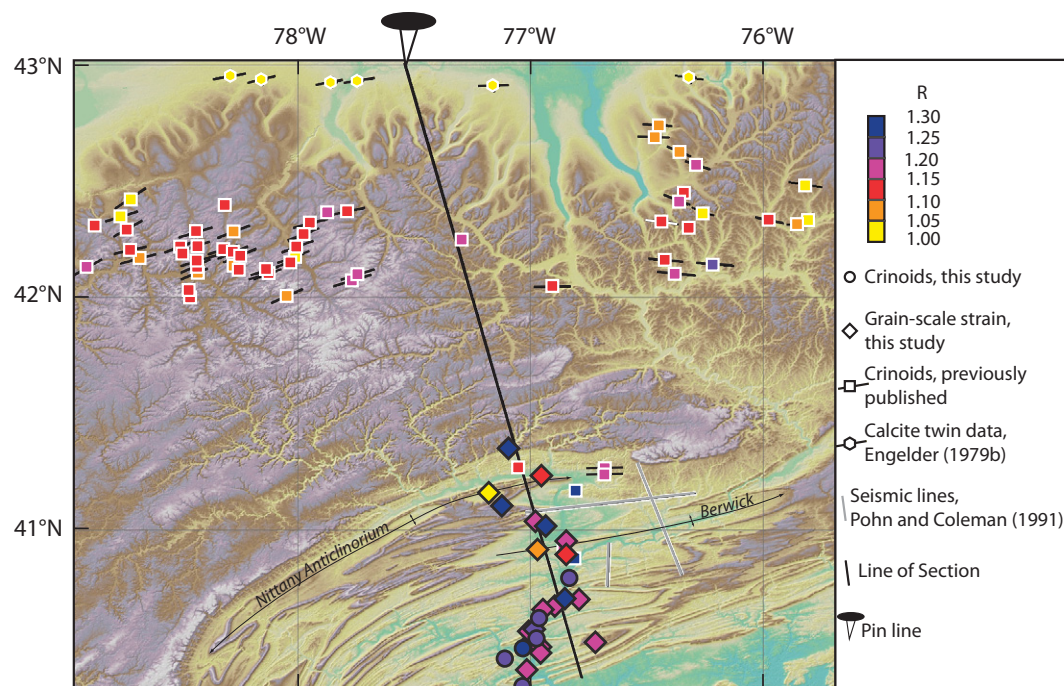
Figure 5. Shaded relief map of the study area and surrounding regions showing the distribution and magnitude of measured finite strain (from Engelder, 1979b; Slaughter, 1982; Geiser and Engelder, 1983; Nickelsen, 1983; and this study [larger symbols with black outlines]), locations of published seismic lines (Pohn and Coleman, 1991), and the line of cross section in Plate 1.
