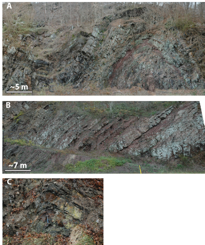
Figure 9. Outcrop-scale structural styles along roadcuts. (A) The most extensive example of third-order folds observed in the study area. Here, folds have wavelengths of tens of meters. (B) Homoclinally dipping package of Devonian Irish Valley Member exposed in a roadcut along the west shore of the Susquehanna River. Uniform dipping sequences are typical throughout the study area. (C) Mesoscale anticline in the Devonian Tonoloway Formation. Note the well-developed wedge faults in the core of the fold in the competent beds and extensive axial planar cleavage in the less competent units. Note hammer for scale.
