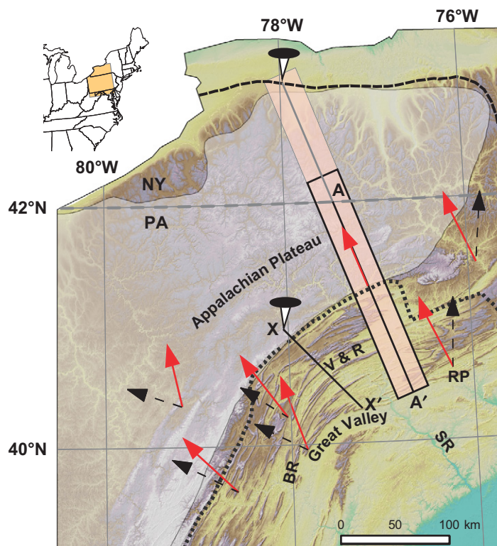
Figure 1. Shaded relief map of the Pennsylvania salient and surrounding region showing the subsurface extent of Silurian salt horizons (light blue shaded region) (modified after Davis and Engelder, 1985); northern limit of layer-parallel shortening (dashed line, after Geiser and Engelder, 1983); position of the Alleghany front (dotted line); compilation of tectonic transport vectors (red arrows—early transport direction; black arrows—late transport direction) from Gray and Stamatakis (1997). Shaded red box—study area; heavy black outlined box—extent of Figure 4; bold line labeled X–X'—line of section shown in Figure 2; bold line labeled A–A'—line of section shown in Plate 1. BR—Blue Ridge; RP—Reading Prong; SR—Susquehanna River; V&R—Valley and Ridge; NY, PA—New York, Pennsylvania. Note that the line of section parallels the transport direction along the axis of no rotation of the maximum shortening direction.
