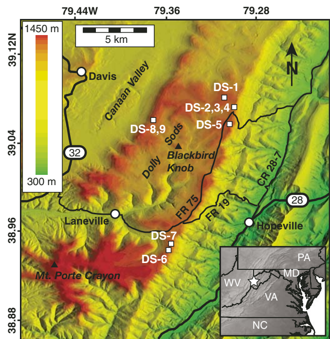
Figure 1. Shaded relief map constructed from 30 m digital elevation model of the Dolly Sods area, West Virginia, showing sampling locations DS-1 to DS-9 and major topographic features. Inset shows general site location. PA—Pennsylvania; MD—Maryland; WV—West Virginia; VA—Virginia; NC—North Carolina.
