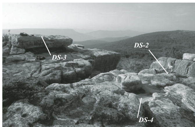
Figure 2. Photograph looking southeast over the edge of the Dolly Sods upland. Shown are sample collection locations for samples DS-2 (lower bedrock surface, note person for scale), DS-3 (upper bedrock surface with well-developed weathering pits), and DS-4 (residual quartz clasts).
