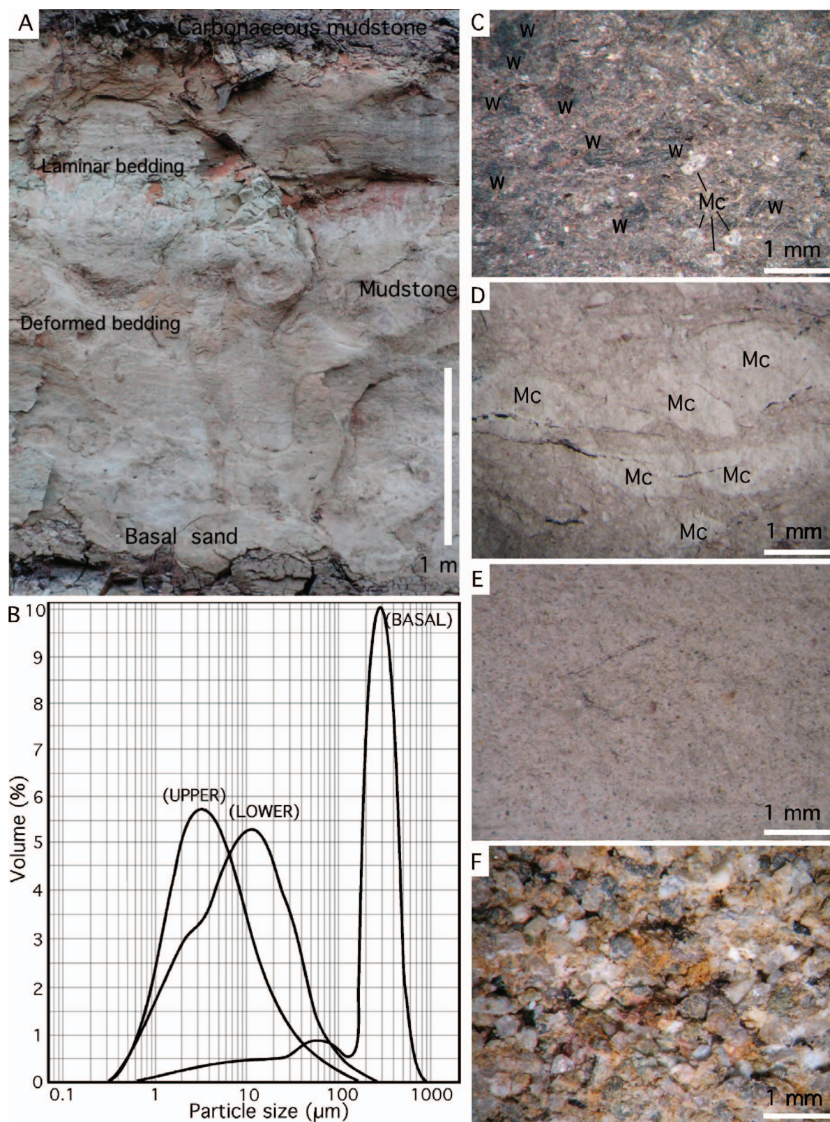
FIGURE 6 —Volcanic mudstone flow units in Red Gate section, WWU 2138. A) Flow unit #3 showing an upward-fining grain size trend and different layers within the flow unit. Irregularities on the basal surface result from differential deformation of underlying sediment. Circular structures in the middle of the flow result from internal deformation of moving sediment. B) Representative sediment grain size distribution (Malvern laser spectrometry) of samples within a flow unit. C) Bedding plane view of plant scrap-rich unit at top of flow unit containing low-density particles (mostly wood, =W) and small mud clasts (=Mc, white). D) Bedding plane view of mud clast-rich layer below capping plant-rich layer with white mud clasts (=Mc) set in tan-colored mudstone matrix. Irregular outline of mud clasts suggests tearing and fragmentation during transport. E) Silt-rich mudstone from middle of flow unit, with dispersed sand-sized grains visible. F) Sand layer at base of flow unit with dominant mode of medium-size sand grains.
