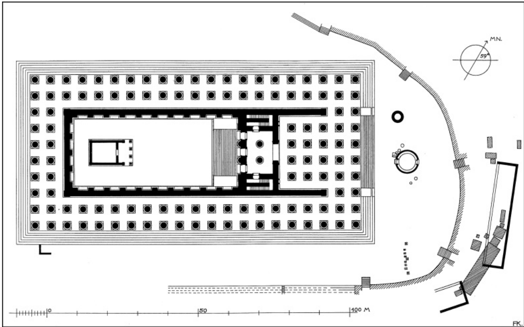
90. Plan of the temple of Apollo, Figure 89. A sacred grove of laurel trees stood within its vast, 71 \times 150 ft. ( 21.7 \times 45.4 m), open-air inner courtyard, concealing a smaller Ionic temple measuring 28 \times 47.7 ft. ( 8.6 \times 14.5 m) and 35 ft. (10.4 m) high. This housed the archaic cult statue of Apollo by Kanachos of Sikyon, taken by the Persians in 494 but returned by Seleukos I.
