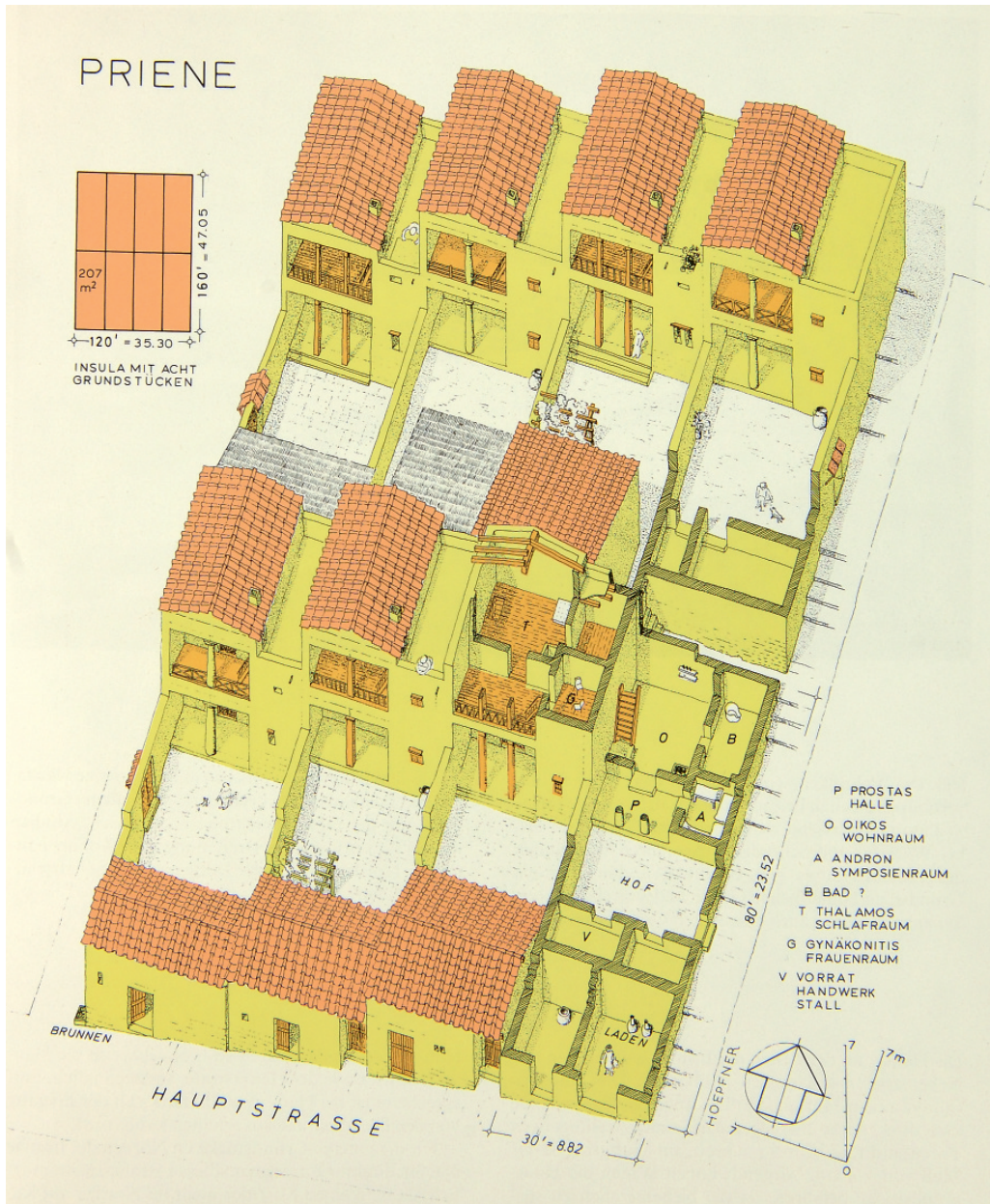
12. City block and house at Priene, ca. 300. Each block, measuring 120 \times 160 Attic ft., accommodated eight building plots, or parcels, each of 30 \times 80 ft. (2,400 sq. ft.): a very democratic arrangement. The large and sturdy stone houses were spacious, cool in the summer, and draft resistant in the winter. Many featured an internal courtyard overlooked by a stately pastas/prostas , or vestibule, fronted by a short verandah. Richer interiors boasted pebble floor mosaics; frescoed faux-marble panels, moldings, and colonnades; and the occasional marble statuette.
