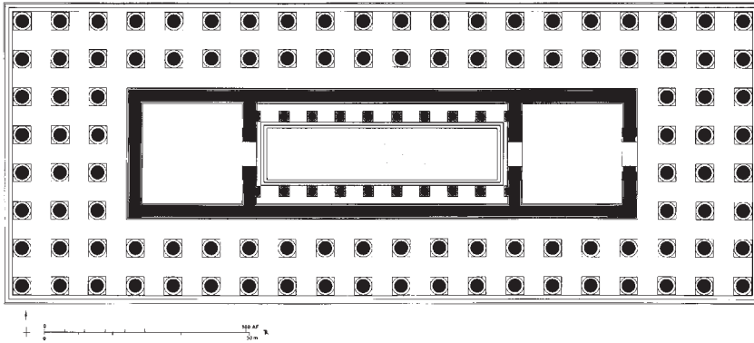
48. Temple of Olympian Zeus at Athens, ca. 175–164 (columns, capitals, and architraves), Augustan and Hadrianic (the remainder). Funded by King Antiochos IV of Syria, designed by the Roman architect Decimus Cossutius, and made entirely of marble, it replaced an unfinished Doric limestone temple begun by the tyrant Peisistratos in the 530s. At 135 \times 354 ft. ( 43 \times 110 m), it equals an American football field in size. Like its archaic predecessor, it had a double colonnade (triple on the façades) of 8 \times 20 columns, 104 in all, perhaps ultimately inspired by the forests of columns inside many Egyptian temples. H of column 55 ft. 5 in. (16.89 m).
