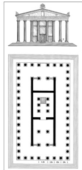
91. Reconstructed view, elevation, and plan of the Ionic temple and altar of Artemis Leukophryene at Magnesia-on-the-Maeander, designed ca. 200 by Hermogenes of Alabanda. Measuring 103 \times 190 ft. ( 31.6 \times 57.9 m) on the stylobate and obsessively
