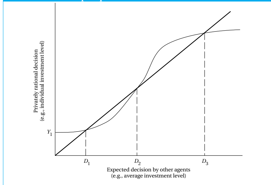
FIGURE 4.1 Multiple Equilibria
