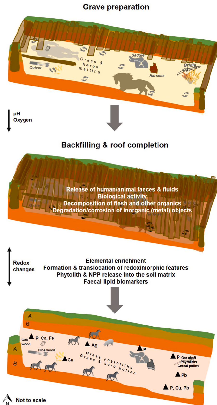
Fig. 10. Simplified model of grave establishment and post-depositional processes.
