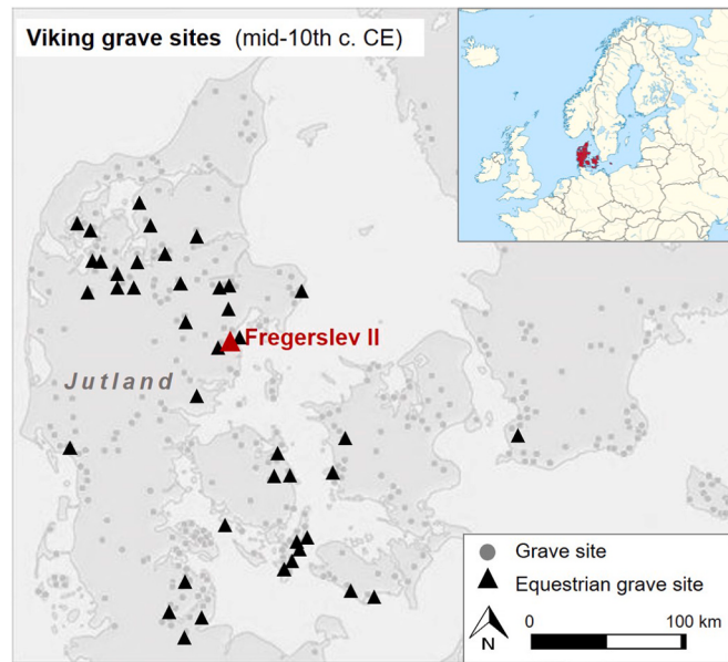
Fig. 1. Viking grave sites contemporary to Fregerslev II. Base map adapted from denstoredanske.dk ; distribution of equestrian graves from Peder-sen (2014) .
