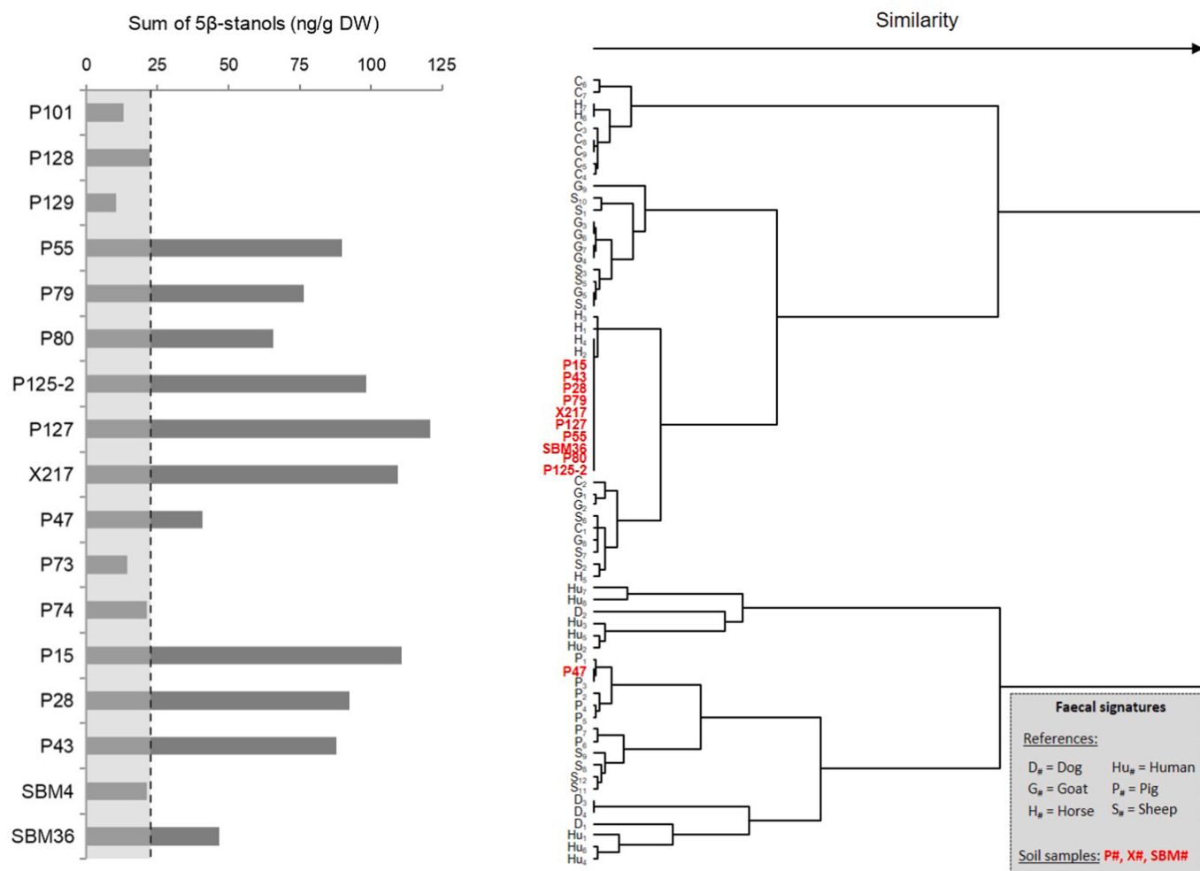
Fig. 8. Faecal lipid biomarkers: a. left, sum of 5β-stanols; right, hierarchical cluster; b. left, fragmentograms from two different samples (P80 with a suggested horse signature and p47 with a suggested pig signature); right, partial chromatograms of a steroid standard mixture (top) and a reindeer faeces lipid extract used as internal reference (second from the top). Fragmentograms of the lipid extract from sample P15. TIC = partial total ion current analysed in SIM mode. IS 2 = injection standard (5α-Cholestane). IS 1 = recovery standard (5β-Cholan-24-ol). Greyed compound names display unstudied steroids. Fragmentogram colours are purely graphical. (For interpretation of the references to colour in this figure legend, the reader is referred to the Web version of this article.)
