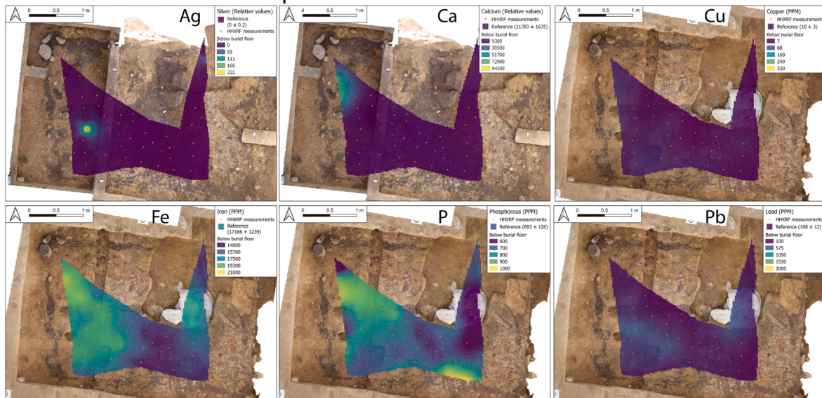
Fig. 5. Elemental concentrations of Ag, Cu, Fe, P, and Pb in the burial floor layer and the soil below it.
