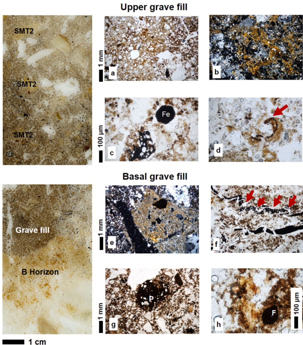
Fig. 6. Microstructure and key pedofeatures of the grave fills. Left, scans of the thin sections from the grave fill and B horizon; right micrographs: a. structure and porosity exhibiting different degree of iron impregnation, PPL (plane polarized light); b. mix of different soil microfabric types, XPL (crossed-polarized light); c. iron typic nodule (Fe), PPL; d. iron-manganese hypocoating (red arrow), PPL; e. mix of different soil microfabric types, XPL; f. horizontal distribution of plant remains with red arrows indicating potential direction of compression, PPL; g. potsherd (P), PPL; h. amorphous organic matter and fungal spore (F), PPL. (For interpretation of the references to colour in this figure legend, the reader is referred to the Web version of this article.)
