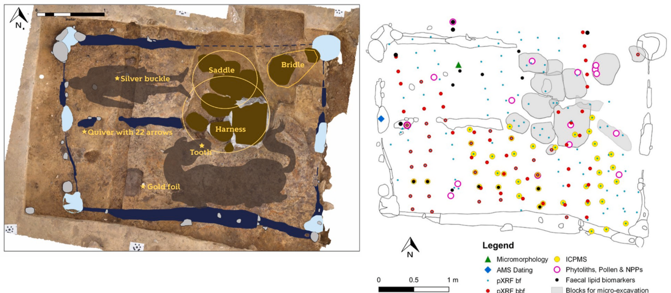
Fig. 3. Left: Aerial photograph of the 2017 trench showing the location of main finds and interpretative model of the grave; right: plan of the trench showing the sample locations.
