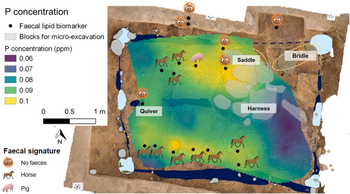
Fig. 9. Distribution of faecal lipid biomarker and P concentration.
