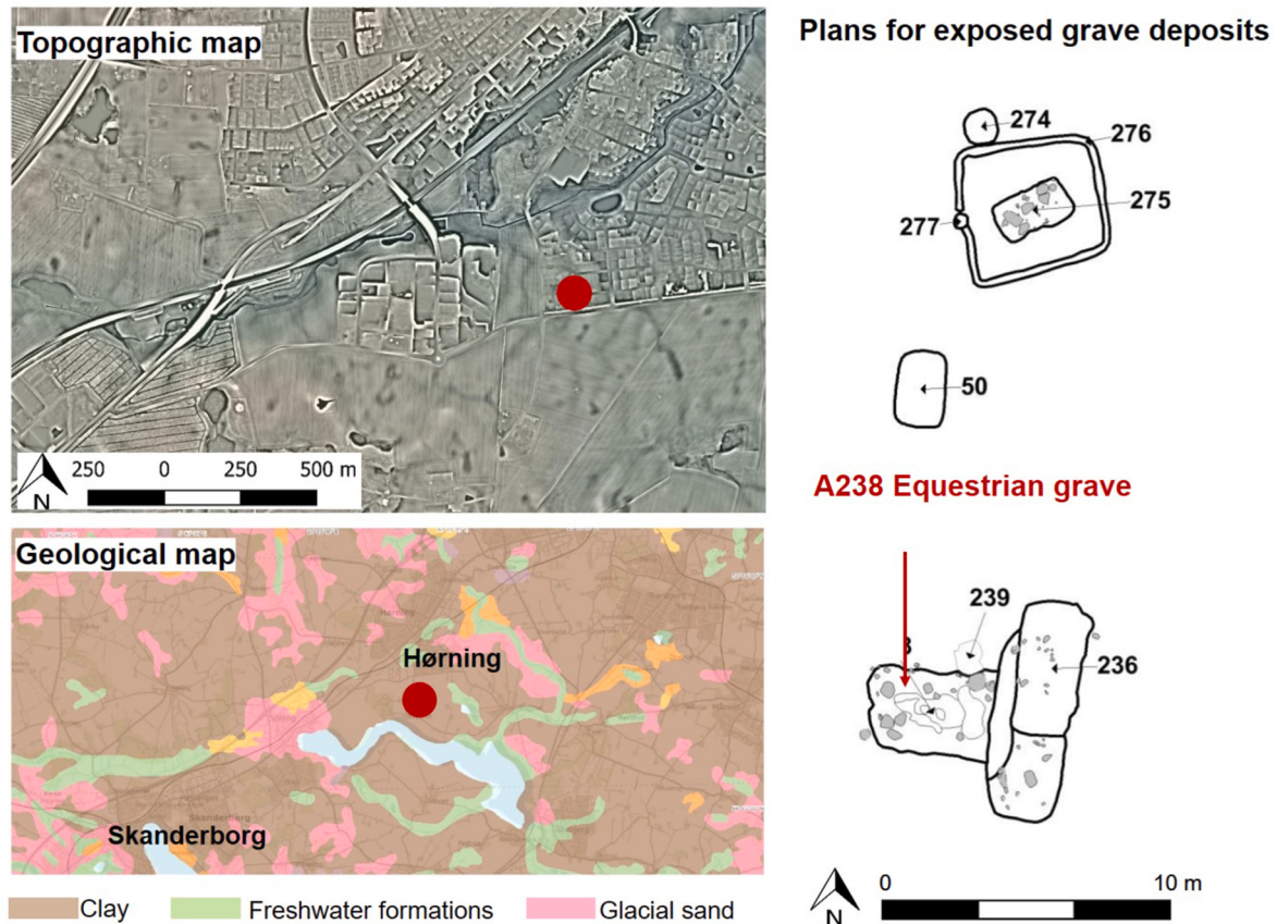
Fig. 2. Location of Fregerslev II; digital elevation model with a residual relief model ( Stott et al., 2019 ); geological soil type map (after GEUS); the three graves recorded at Fregerslev II (adapted from Bagge, 2016 ).
