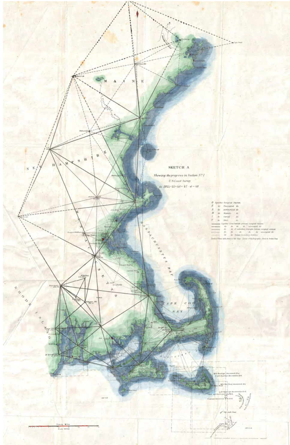
Figure 3-17: A map of the triangulation survey network established the northeastern coast of the United States of America in the early 1800s. Each leg of the triangles, shown here as a single line, is in turn a triangulation survey. This nested triangulation provides reinforcing measurements, thereby increasing the accuracy of the surveyed positions (courtesy NOAA).
